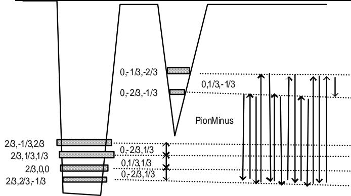
Figure 17. Pion Minus Coherence.
