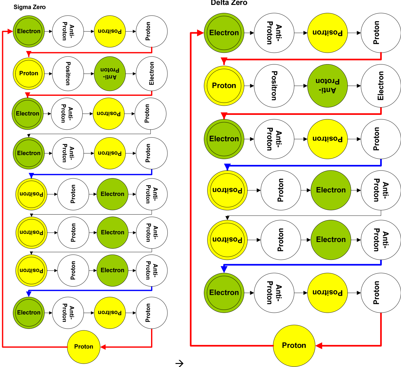
Gamma Ray Figure 26. Sigma Zero decay diagram.
