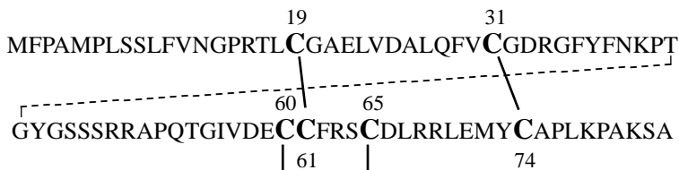
Scheme 2. Amino acid sequence and disulfide bond linkage of LR 3 IGF-I.
