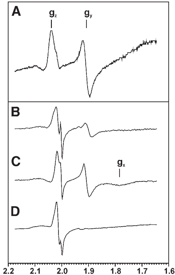
Fig. 3. EPR spectra from E. coli cell membranes containing PetC2 ( B ) and PetC3 ( C ). ( A ) Shows the EPR signal from the isolated and in vitro reconstituted PetC1 protein ( I3 ), and in ( D ) a control of E. coli cell membranes is shown. The positions of the g_{y,z} -values are indicated in ( A ). The g_x -value could only be determined accurately for the PetC3 protein ( C ).
