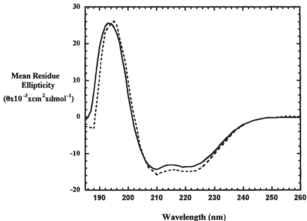
Fig. 3. CD spectra of glycerol facilitator solubilized in 10 mM sodium phosphate buffer containing 10 mM sodium chloride and detergent at 25°C. (—) GF dissolved in 150 mM SDS at pH 7.6; (---) GF dissolved in 30 mM DM at pH 7.0.
