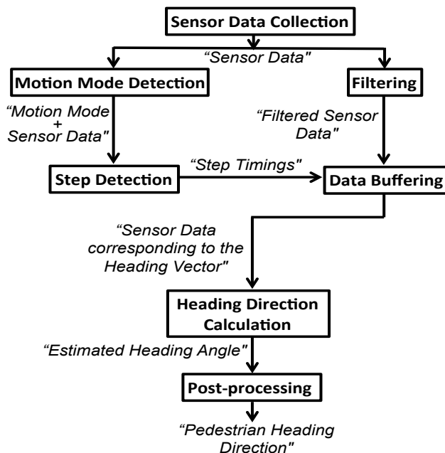
Figure 5.1: The flow diagram of the WalkCompass application.
