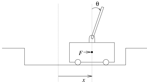
Figure 7.3: The cart-pole system.
