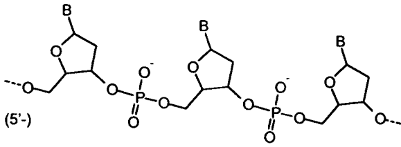
DNA
