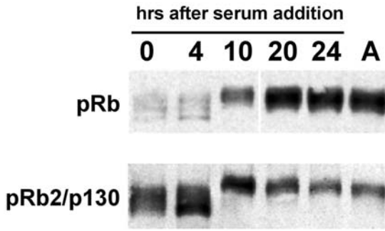
Fig. 1. Western blot showing phosphorylation kinetics of pRb and pRb2/p130 in T98G human malignant glioma cell line. Cells were arrested in G 0 by serum deprivation for 48 h, then serum was added and the synchronized cells were allowed to proceed through the cell cycle and collected after 4, 10, 20, and 24 h. A, asynchronous cell population.
