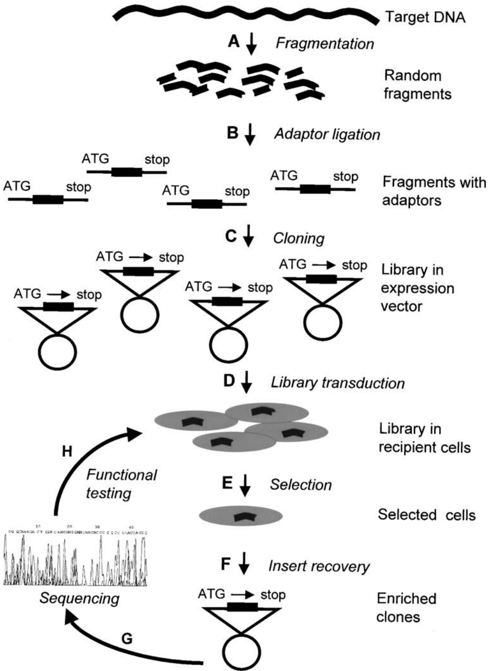
Fig. 1. General scheme of GSE selection. See text for details.
