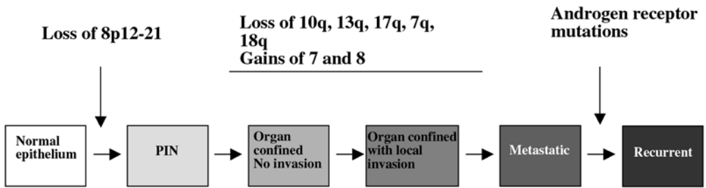
Fig. 2. Progression model of prostate cancer. The events are not well defined. Androgen receptor is probably always needed for the growth of the cancer cells. However, mutations give advantage to the cancer cells at advanced disease and during androgen depletion.
