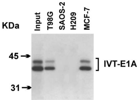
Fig. 2. Autoradiography of the analysis by SDS-PAGE (10%) of coimmunoprecipitation of IVT-E1A bound to pRb from different cell lines. [ 35 S]-labeled IVT-E1A was preincubated with unlabelled cell lysates prepared from T98G, SAOS2, H209, MCF-7 cell lines and coimmunoprecipitated using the pRb-specific C36 monoclonal antibody. Input, an equivalent amount of [ 35 S]-labeled IVT-E1A was immunoprecipitated using the E1A specific M76 monoclonal antibody. Left ordinate, molecular-weight marker migration distances.
