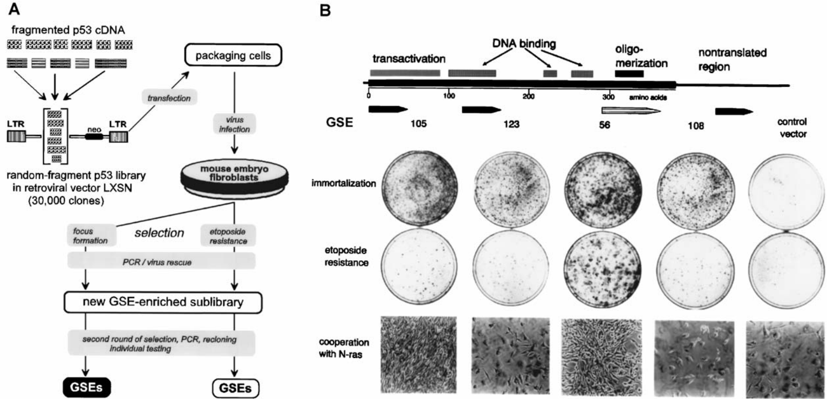
Fig. 2. Scheme of GSE selection from p53 (A) and comparison of biologic activity of GSEs derived from different portions of p53 cDNA (B) (reproduced from ref. 20). See text for details.
