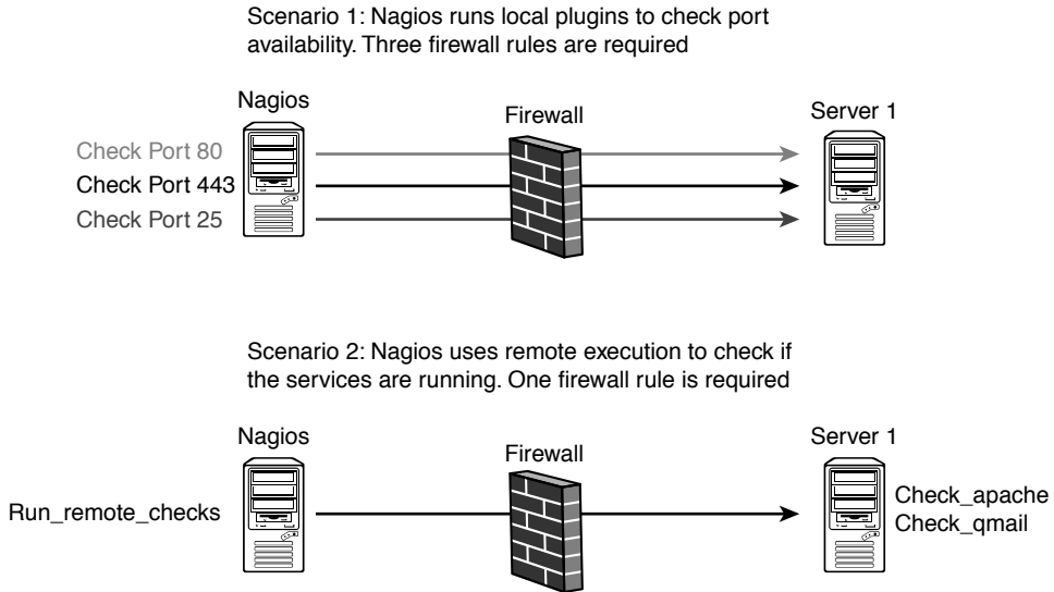
Figure 1.3 When used correctly, remote execution can enhance security by minimizing firewall ACLs.
