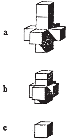
FIGURE 6. Step by step construction of a 4-D cube (Tesseract) by folding seven 3-D cubes (cubes) out of the source space (space) around their boundaries (edges). Compare Fig. 6a with Salvador Dali's painting "Crucifixion (Corpus Hypercubus)" in the New York metropolitan Museum as, for instance, reproduced in. (17)
