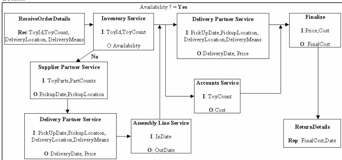
Figure 1: Sample Web Process 1 ( getOrderPriceAndDeliveryDate )
