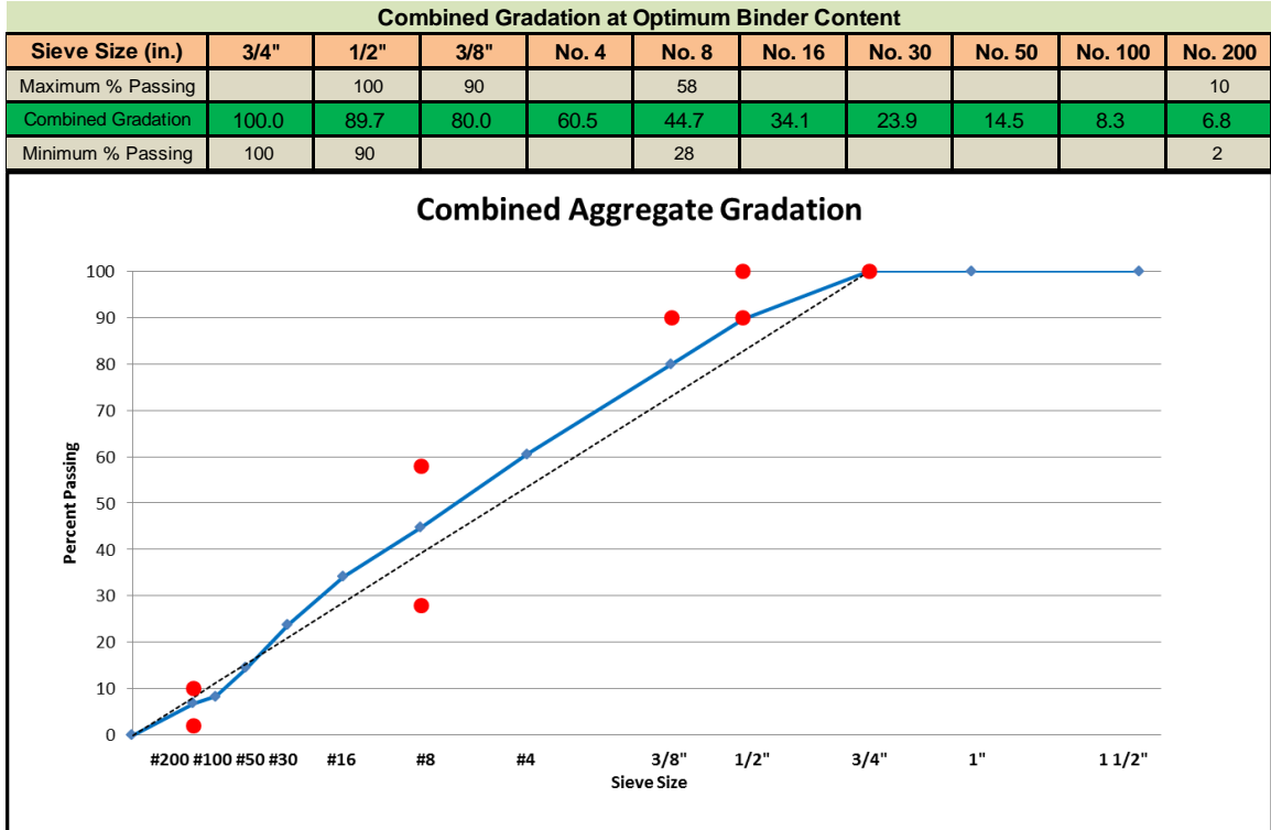
Figure F21: Combined Aggregate Gradation – 50% Traditional RAP-C Mix Design
