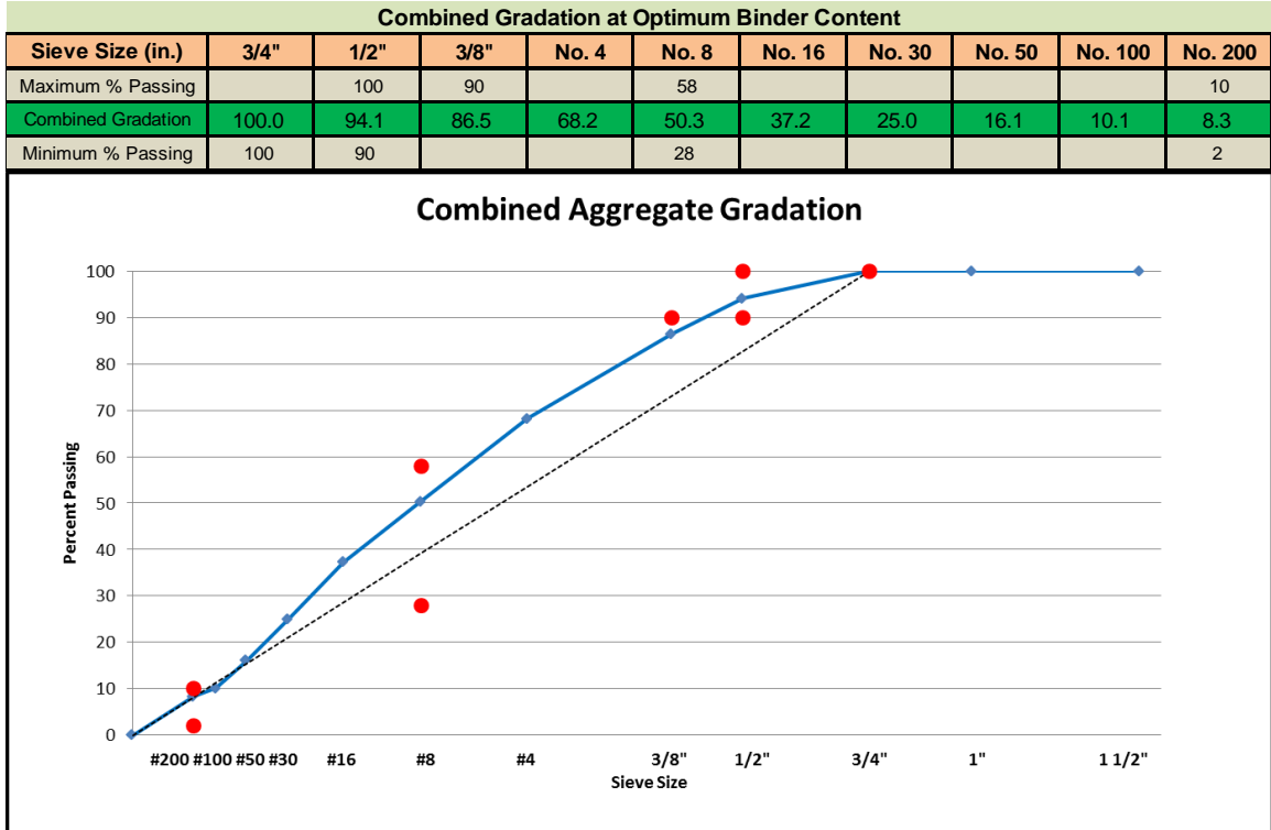
Figure F15: Combined Aggregate Gradation – 50% Fractionated RAP-B Mix Design
