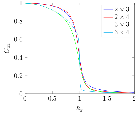
Fig. 5.13 C_{\text{tri}}(\rho_{ABC}) for different values of h_y . The horizontal axis is the magnetic field h_y . The vertical axis is C_{\text{tri}}(\rho_{ABC}) for the ground state of H^{\text{toric}}(\mathbf{h}) .
