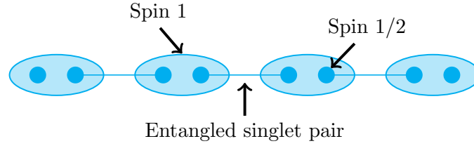
Fig. 10.1 Projected entangled pair structure of the AKLT wave function.
