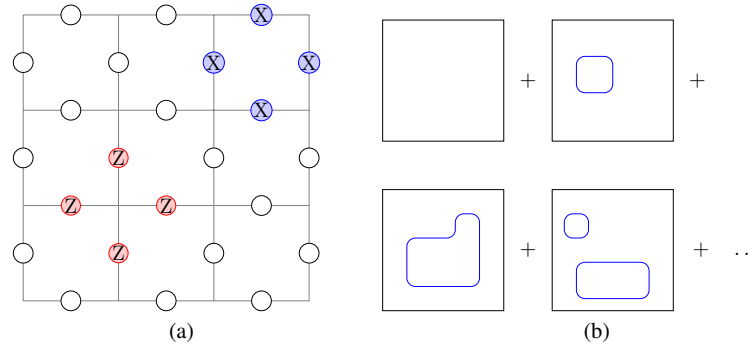
Fig. 5.6 Hamiltonian (a) and ground state wave function (b) of the toric code model.
