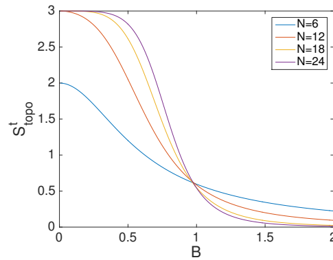
Fig. 5.25 S_{\text{topo}}^t the ground state of H_{\text{ZXZX}}(B) . The horizontal axis is the magnetic field B . The vertical axis is S_{\text{topo}}^t for the ground state of H_{\text{ZXZX}}(B) . For N = 6 , the maximum value of S_{\text{topo}}^t is 2 due to that the system size is too small.
