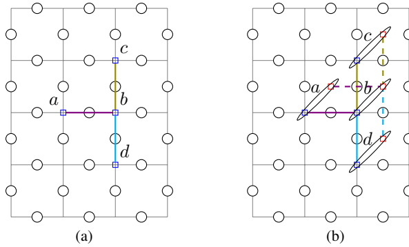
Fig. 6.21 (a) Type- e particles hopping among the four sites a, b, c, d . (b) Type- ε particles hopping among the four sites a, b, c, d .
