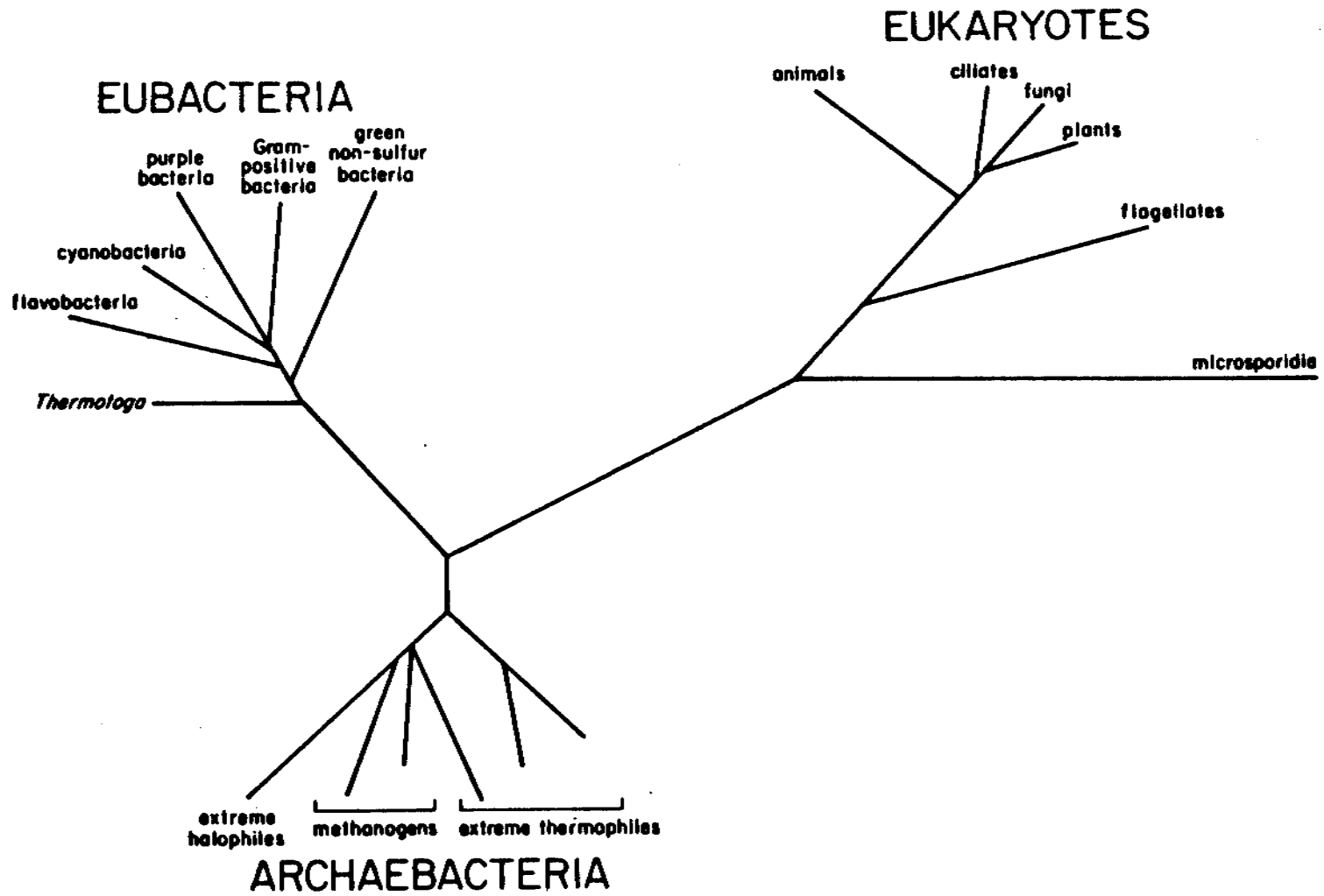
FIGURE 2-1. Universal phylogenetic tree determined from rRNA sequence comparisons (Woese, 1987).
