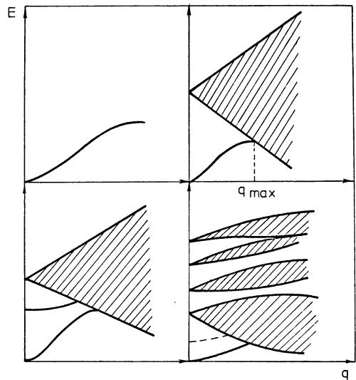
Figure 1: Schematic diagrams of excitation spectra in four microscopic models of theory of magnetism. Upper left: the Heisenberg model; upper right: the Hubbard model; lower left: the Zener model; lower right: the multiband Hubbard model.
