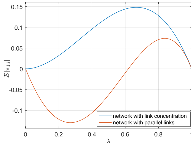
Figure 5 Dependency of a retailer's expected payoff in a small supply chain in a network where both retailers source from the same supplier and a network where they source from two different suppliers.
