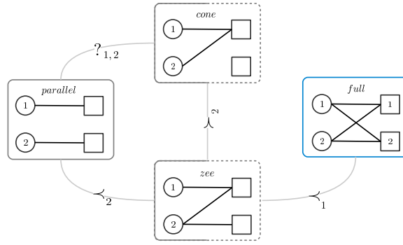
Figure 15 Retailers' preference over networks when \hat{\gamma}_{z2c}(\lambda) < \gamma < \hat{\gamma}_{pz2}(\lambda) . The retailers' expected payoffs are non-negative in the cone network only in the part of the region, and so is the expected payoff of retailer 1 in the zee-shaped network; also the relationship between the cone and the parallel networks change within the region.
