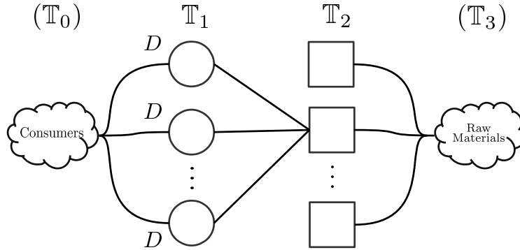
Figure 3 Pure strategy Nash equilibrium in supply chain network formation game without congestion.
