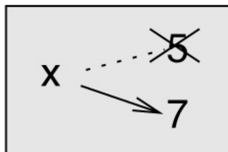
Figure 7-1. State diagram.
