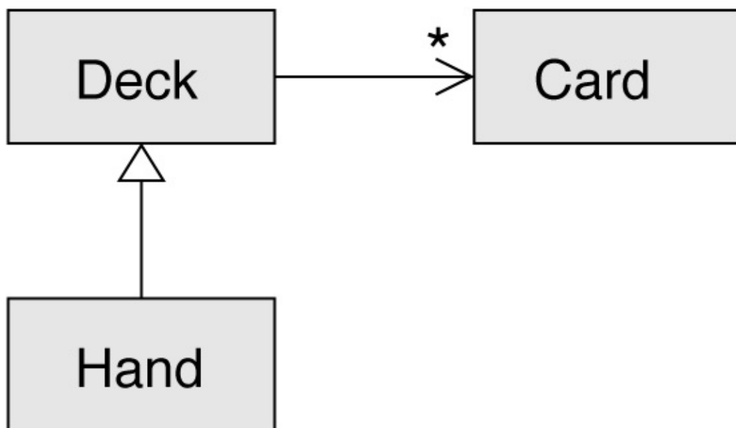
Figure 18-2. Class diagram.
