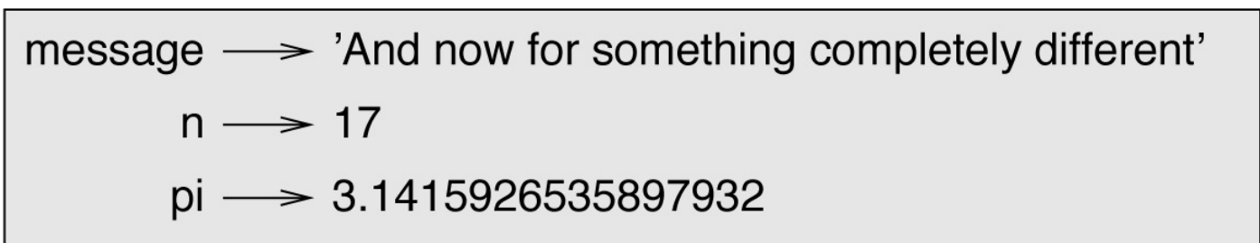
Figure 2-1. State diagram.
