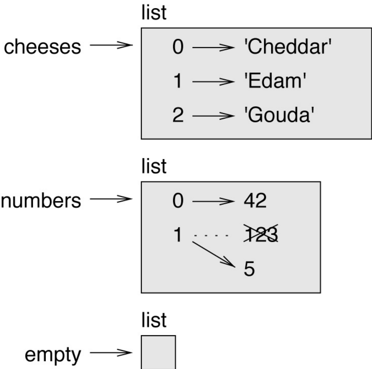
Figure 10-1. State diagram.
