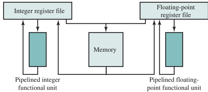
(a) Scalar organization
