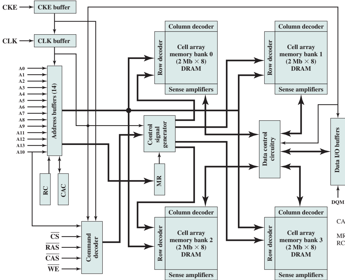
Figure 5.12 Synchronous Dynamic RAM (SDRAM)
