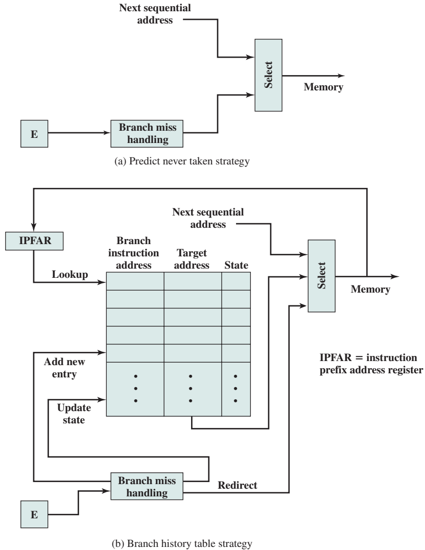
Figure 14.20 Dealing with Branches
