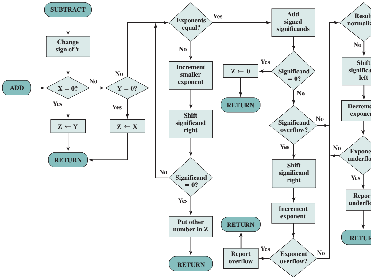
Figure 10.22 Floating-Point Addition and Subtraction ( Z \leftarrow X \pm Y )
