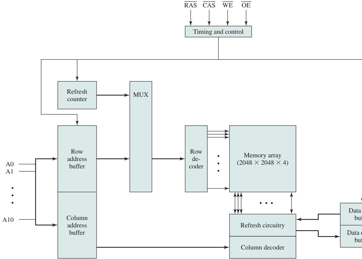
Figure 5.3 Typical 16 Megabit DRAM (4M × 4)
