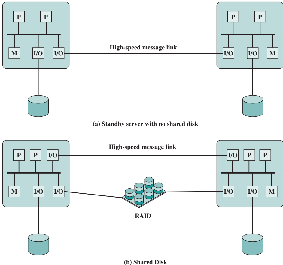
Figure 17.9 Cluster Configurations
