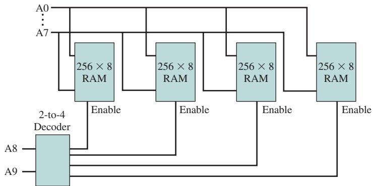
Figure 11.16 Address Decoding
