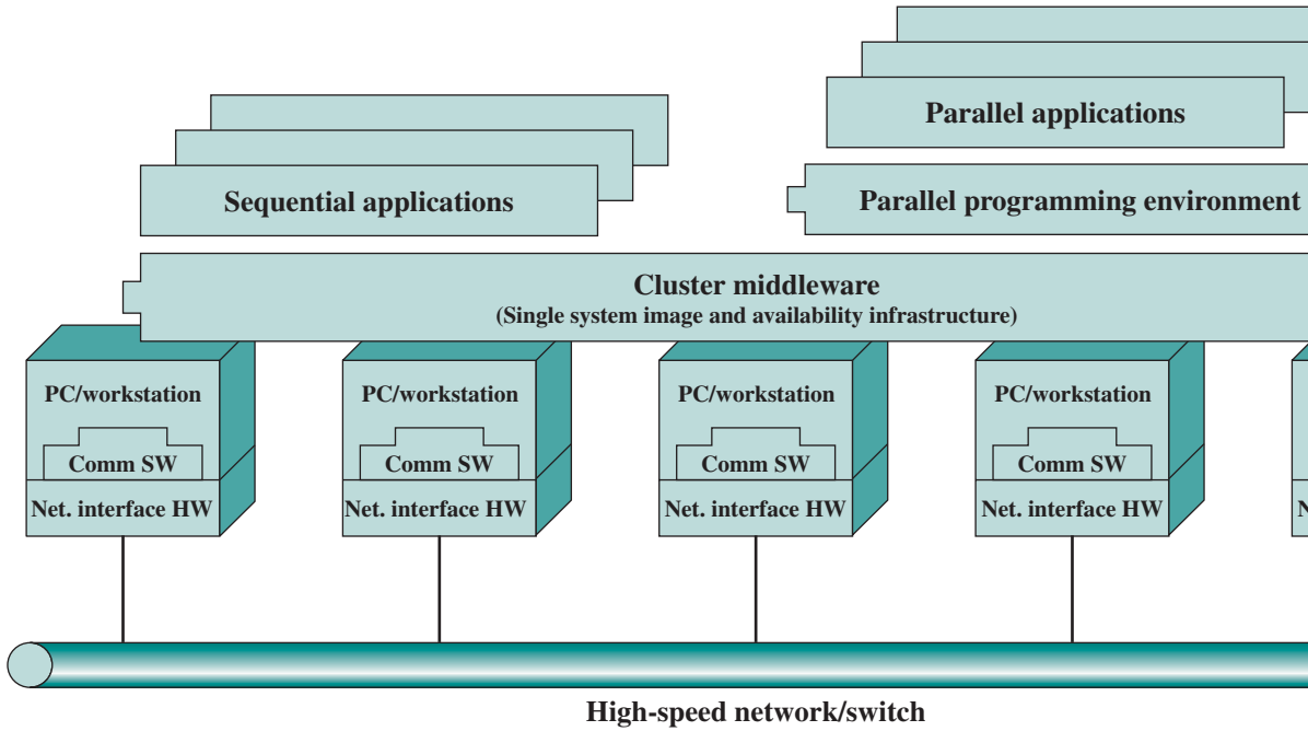
Figure 17.10 Cluster Computer Architecture [BUY99a]
