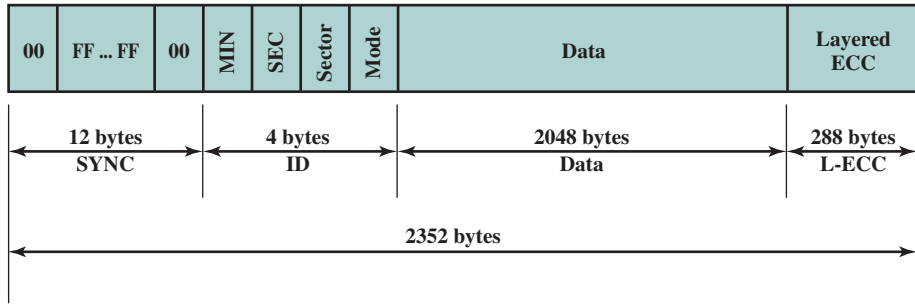
Figure 6.13 CD-ROM Block Format
