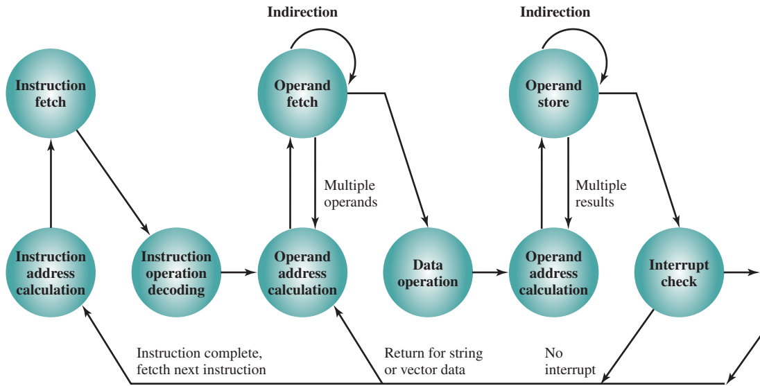
Figure 14.5 Instruction Cycle State Diagram
