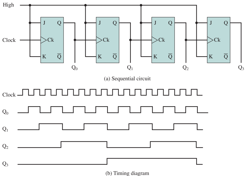
Figure 11.30 Ripple Counter
