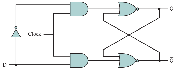
Figure 11.25 D Flip-Flop
