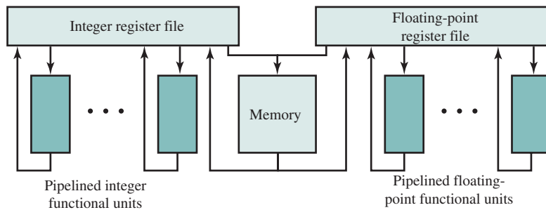
(b) Superscalar organization
