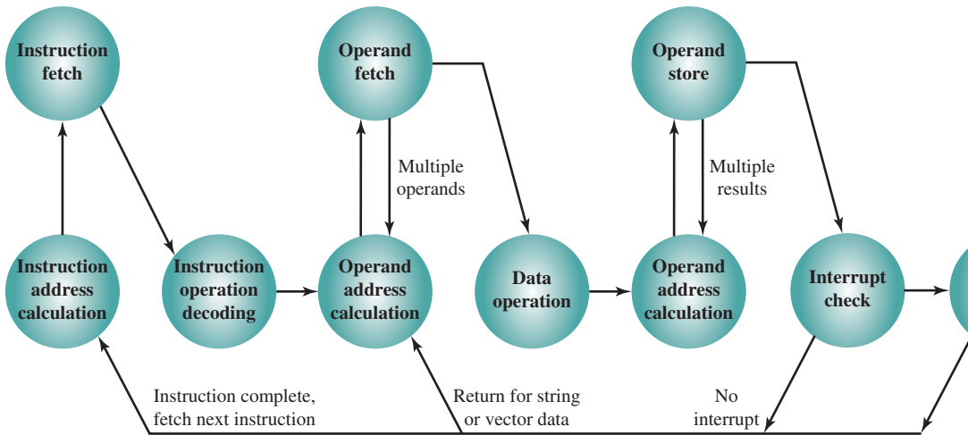
Figure 3.12 Instruction Cycle State Diagram, with Interrupts
