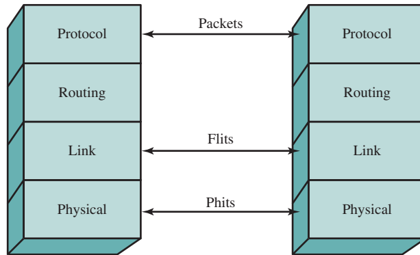
Figure 3.21 QPI Layers
