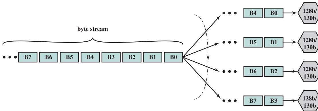
Figure 3.26 PCIe Multilane Distribution
