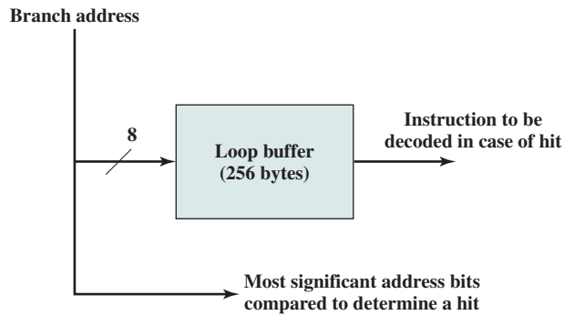
Figure 14.17 Loop Buffer
