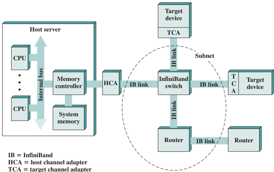
Figure 7.19 InfiniBand Switch Fabric
