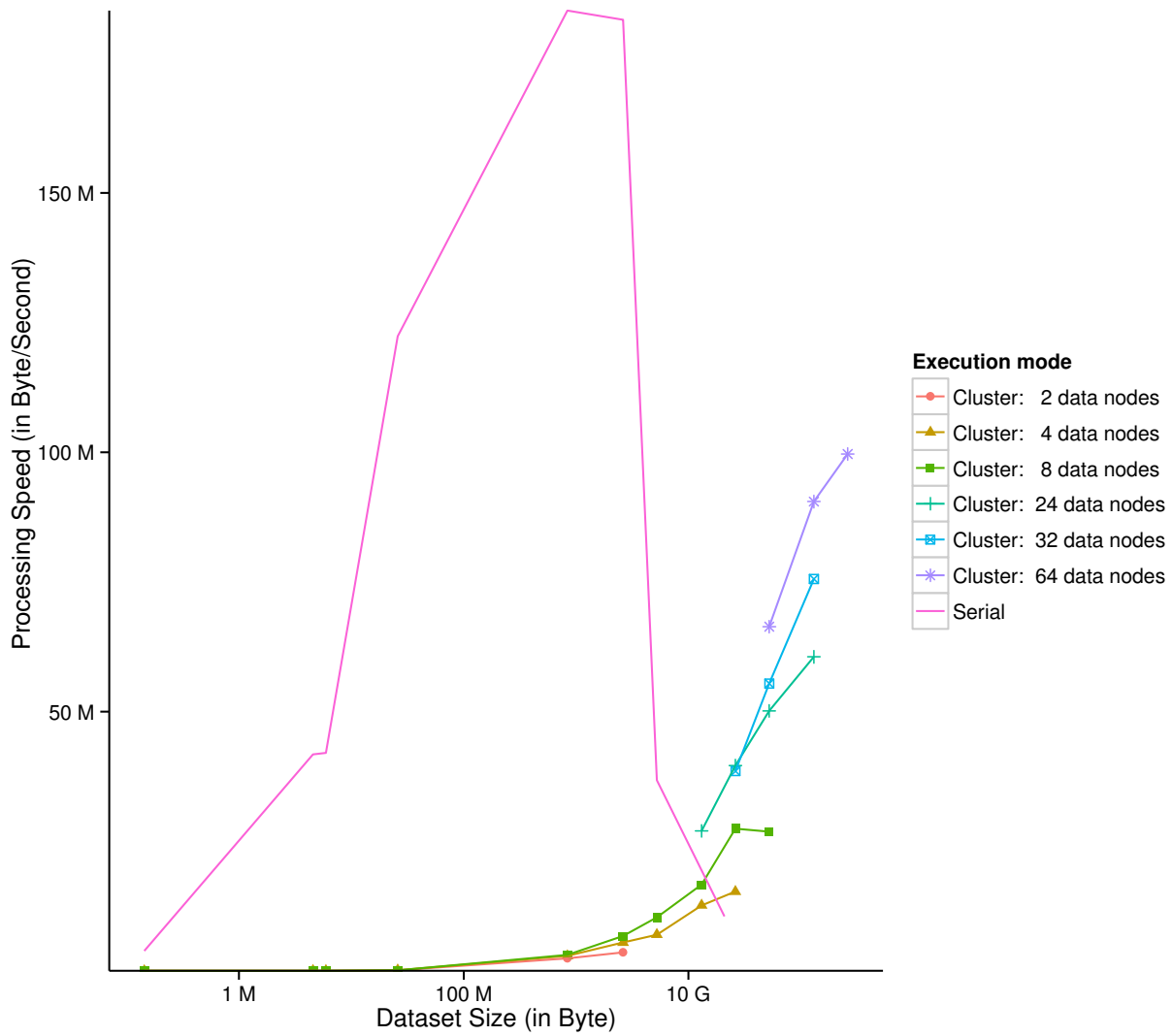
Figure 18: Processing speed of a single ListNet training iteration on various data sets
