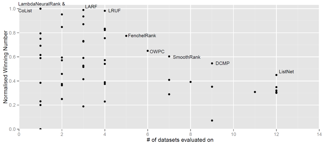
Figure 6: NDCG@3 comparison of Learning to Rank methods
