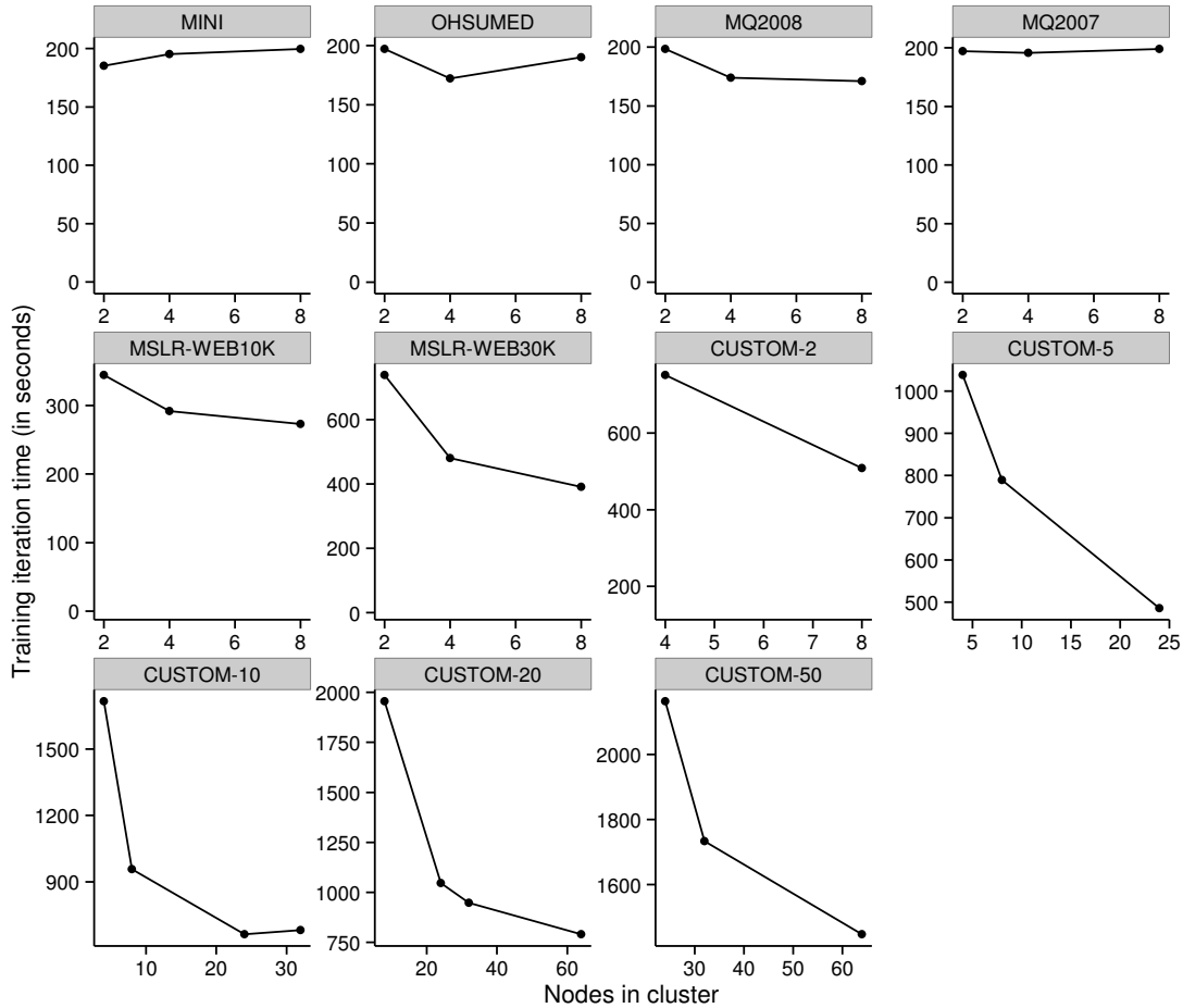
Figure 17: Processing time of a single ListNet training iteration as a function of the number of data nodes in a cluster
