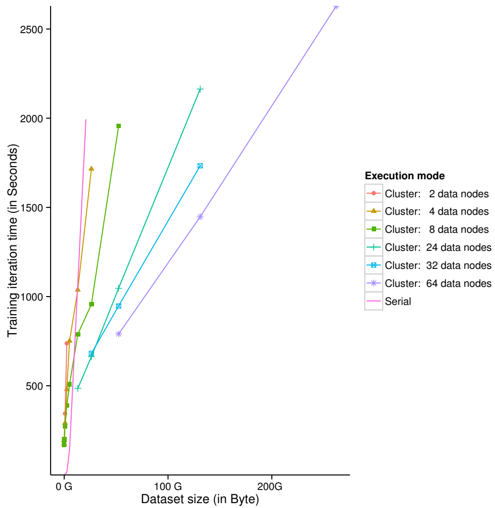
Figure 15: Processing time of a single ListNet training iteration
