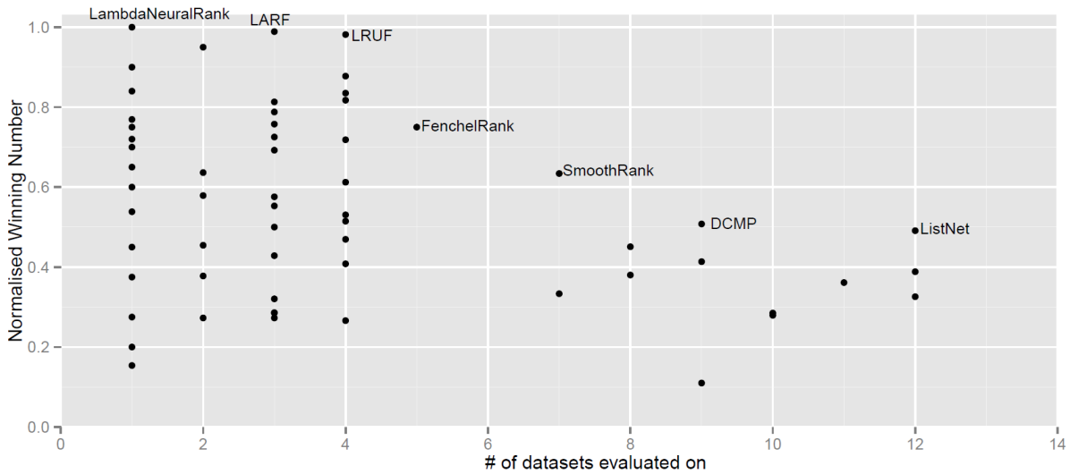
Figure 7: NDCG@5 comparison of Learning to Rank methods
