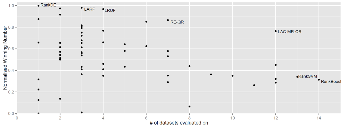
Figure 9: MAP comparison of Learning to Rank methods
