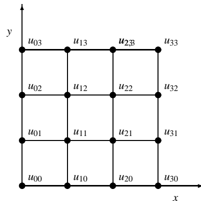
Fig. 10.5 Explicit molecule for n = 3 . The border \delta\Omega defines the boundary condition u(x, y) = g(x, y) .
