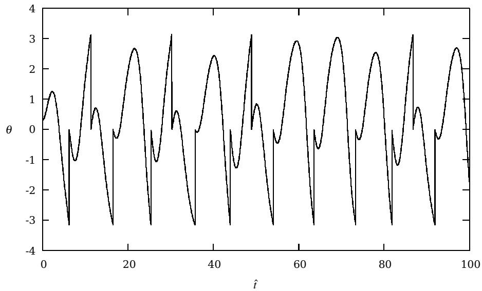
Fig. 8.10 Plot of \theta as function of time \tau with Q=2 , \hat{\omega}=2/3 and \hat{A}=1.35 . The mass of the pendulum is set equal to 1 kg and its length to 1 m. The initial velocity is \hat{v}_0=0 and \theta_0=0.3 . Every time \theta passes the value \pm\pi we reset its value to swing between \theta \in [-\pi, \pi] . This gives the vertical jumps in amplitude.
