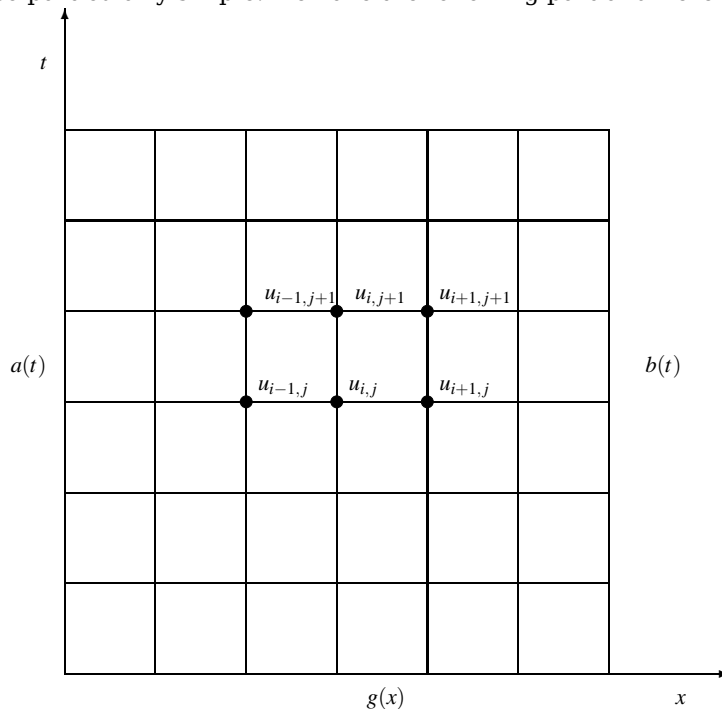
Fig. 10.3 Computational molecule for the Crank-Nicolson scheme.
