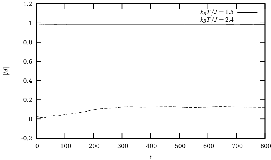
Fig. 13.10 Absolute value of the mean magnetisation as function of time t . Time is represented by the number of Monte Carlo cycles. The calculations were performed with a 100 \times 100 lattice for temperatures k_B T/J = 1.5 and k_B T/J = 2.4 . For the lowest temperature, an ordered start configuration was chosen, while for the temperature close to T_C , a disordered configuration was used.
