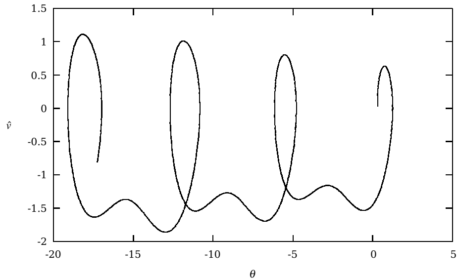
Fig. 8.11 Phase-space curve after 10 periods with Q=2 , \hat{\omega}=2/3 and \hat{A}=1.35 . The mass of the pendulum is set equal to 1 kg and its length l=1 m. The initial velocity is \hat{v}_0=0 and \theta_0=0.3 .
