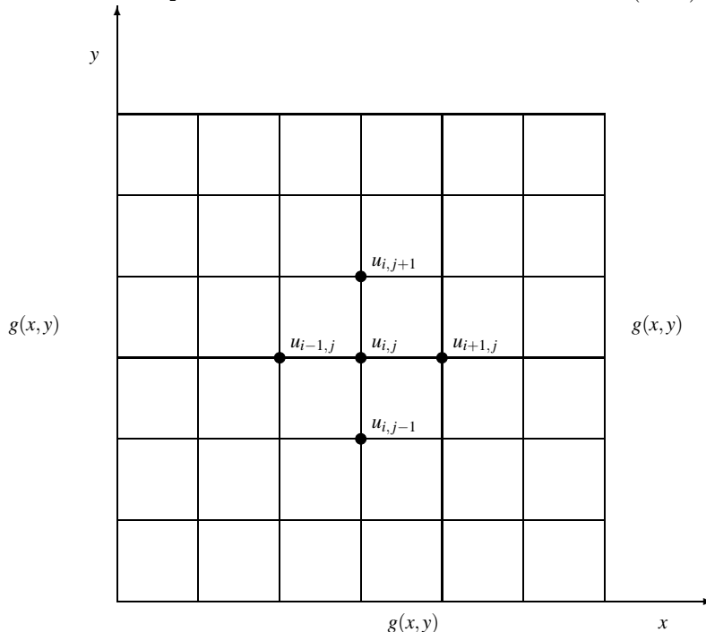
Fig. 10.4 Five-point calculational molecule for the Laplace operator of Eq. (10.13). The border \delta\Omega defines the boundary condition u(x,y) = g(x,y) .
