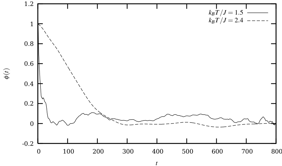
Fig. 13.11 Time-autocorrelation function with time t as number of Monte Carlo cycles. It has been normalized with \phi(0) . The calculations have been performed for a 100 \times 100 lattice at k_B T / J = 2.4 with a disordered state as starting point and at k_B T / J = 1.5 with an ordered state as starting point.
