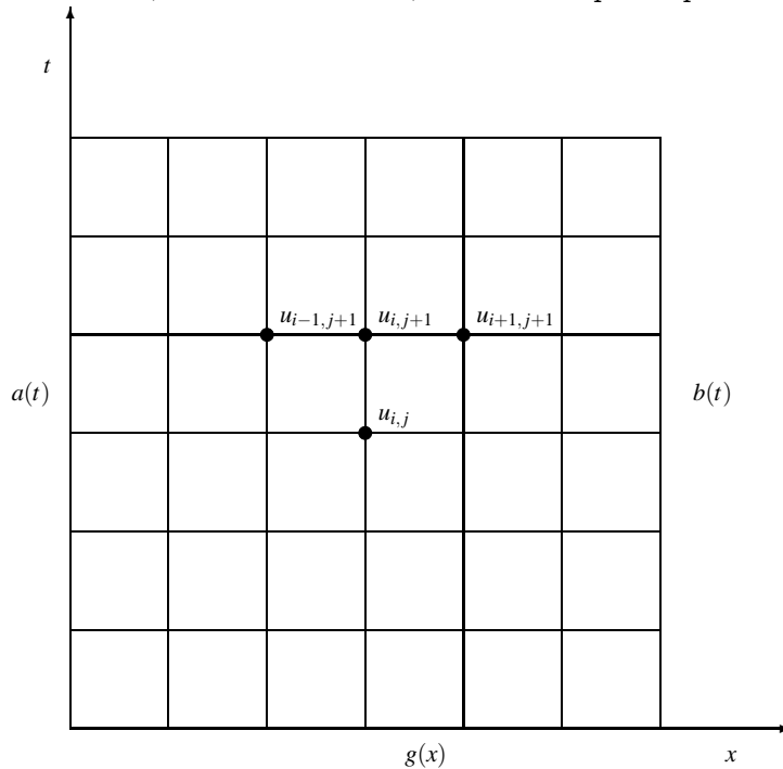
Fig. 10.2 Computational molecule for the implicit scheme.
