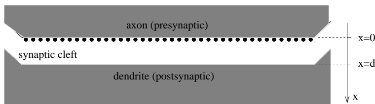
Fig. 10.8 Schematic drawing of the synaptic cleft in our model. The black dots represent neurotransmitter molecules, and the situation shown corresponds to the situation immediately after neurotransmitter release into the synaptic cleft.
