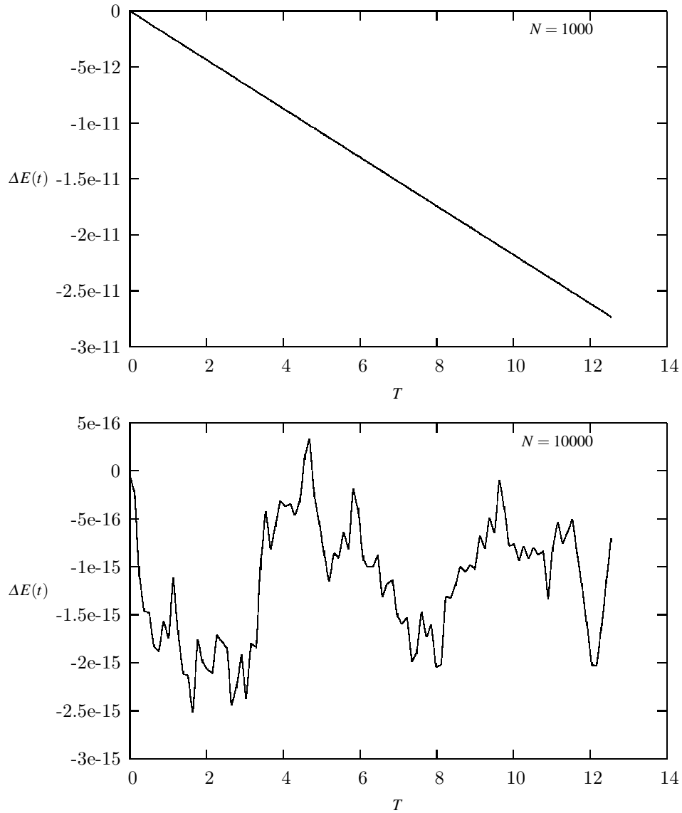
Fig. 8.3 Plot of \Delta E(t) = E_0 - E_{\text{computed}} for N = 1000 and N = 10000 time steps up to two periods. The initial position x_0 = 1 m and initial velocity v_0 = 0 m/s. The mass and spring tension are set to k = m = 1 .
