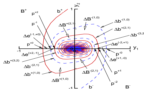
Figure 15: Geometrical spiral showing two special trajectories (the continuous and dashed lines) in the “reduced price”–“velocity” plane (y_1, y_2) that connect exactly the origin y_1 = 0, y_2 = 0 to infinity. This spiraling structure, which exhibits scaling or fractal properties, is at the origin of the accelerating oscillations decorating the power law behavior close to the finite-time singularity. Reproduced from [Ide and Sornette, 2002].
