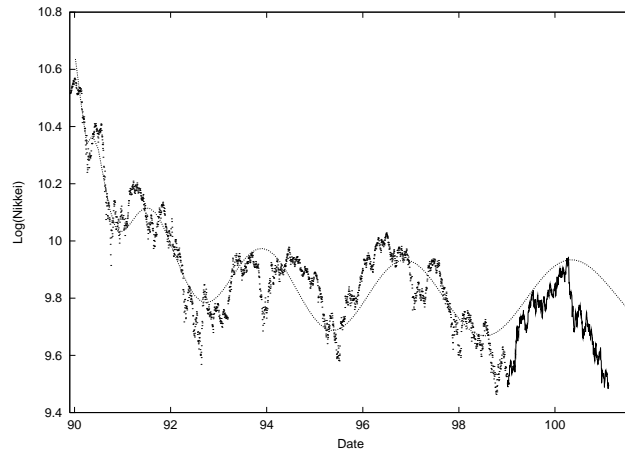
Figure 35: Natural logarithm of the Nikkei stock market index after the start of the decline from 1st Jan 1990 until Feb. 2001. The continuous smooth line is the extended nonlinear log-periodic formula which was developed in [Johansen and Sornette, 1999c] and is used to fit adequately the interval of \approx 9 years starting from 1st Jan 1990. The Nikkei data is separated in two parts. The dotted line shows the data used to perform the fit with formula developed in [Johansen and Sornette, 1999c] and to issue the prediction in Jan. 1999 (see figure 34). Its continuation as a continuous line gives the behavior of the Nikkei index after the prediction has been made. Reproduced from [Johansen and Sornette, 2000b].
