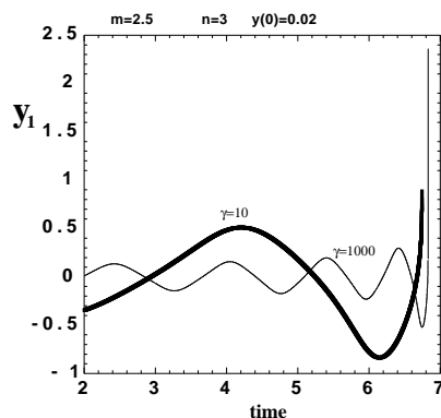
Figure 14: “Reduced price” as a function of time for a trend-following exponent m = 2.5 with n = 3 , \alpha = 1 and with two amplitudes \gamma = 10 and \gamma = 1000 of the fundamental reversal term. Reproduced from [Ide and Sornette, 2002].
