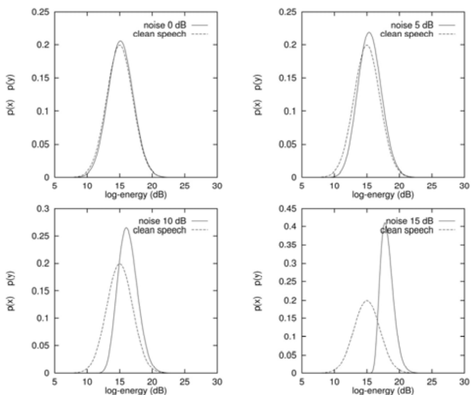
Figure 3. Distortion of the probability distributions caused by additive noise. Clean Gaussian with \mu_x=15\text{dB} and \sigma_x=2\text{dB} . Noise with constant level 0dB, 5dB, 10dB and 15dB
