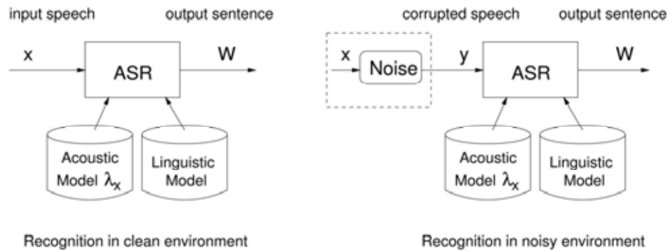
Figure 1. Block diagram of a speech recognition system processing clean or noisy speech with clean speech models
