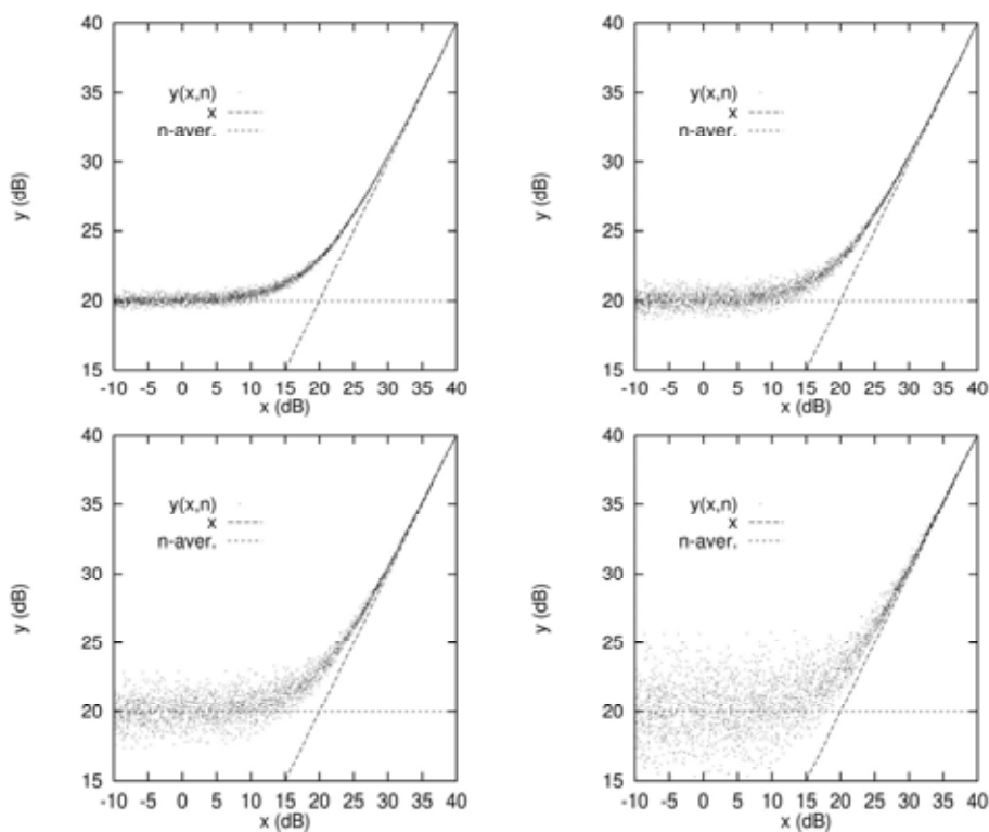
Figure 6. Transformation of clean observations into noise observation when contaminated with a noise with Gaussian distribution with /z_n=20\text{dB} and u_n equal to 0.25dB, 0.5dB, 1dB and 2dB
