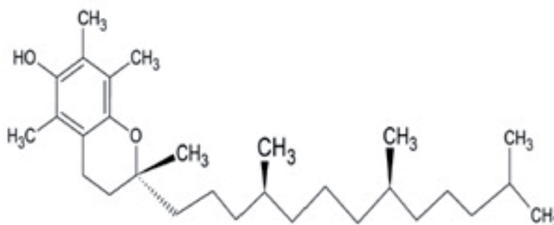
Figure 2. Chemical structure of alpha-tocopherol [4].
