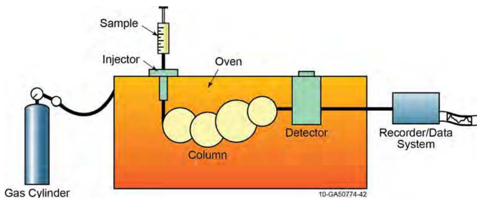
Fig. 1. Schematic view of gas chromatography (Punrattanasin and Spada, 2011)
