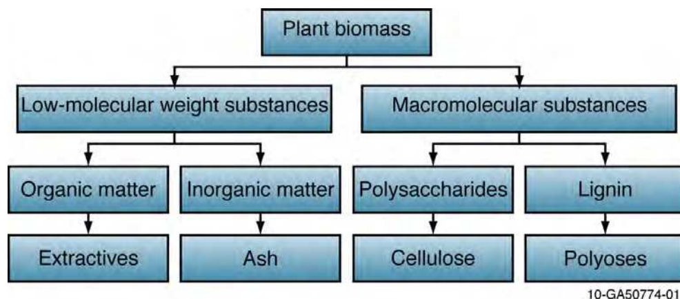
Fig. 2. Plant biomass composition (Mohan et al. 2006)
