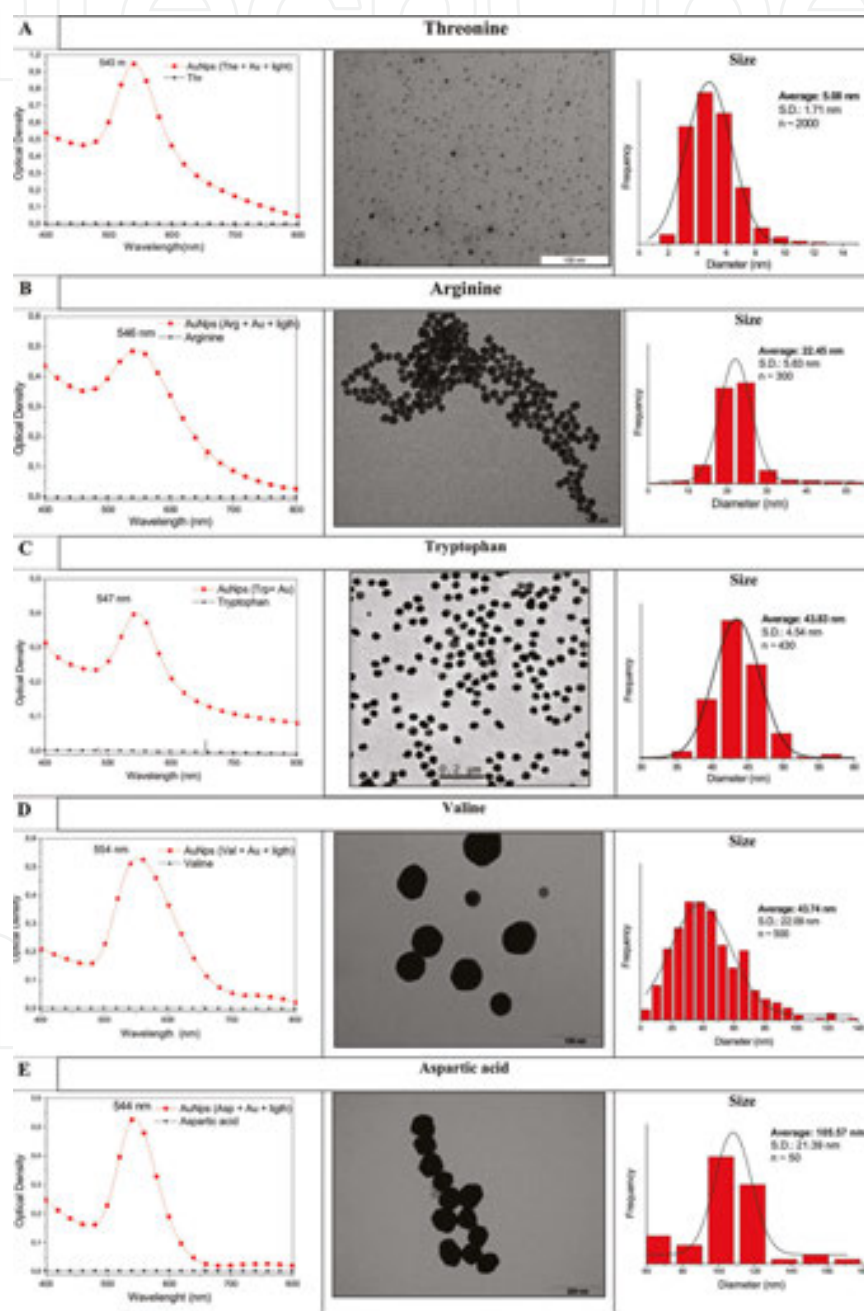
Figure 5. UV-Vis spectra, TEM images, and the average size of the AuNPs prepared with (A) Thr, (B) Arg, (C) Trp, (D) Val, and (E) Asp. Microscopic analyses were performed on a LEO 906E transmission electron microscope (Zeiss, Germany).
