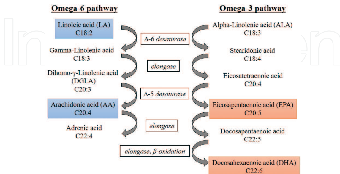
Figure 3. The omega-3 and omega-6 metabolism pathways.
