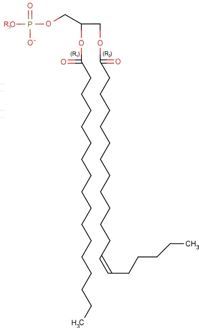
Figure 2. General structure of a phospholipid.
