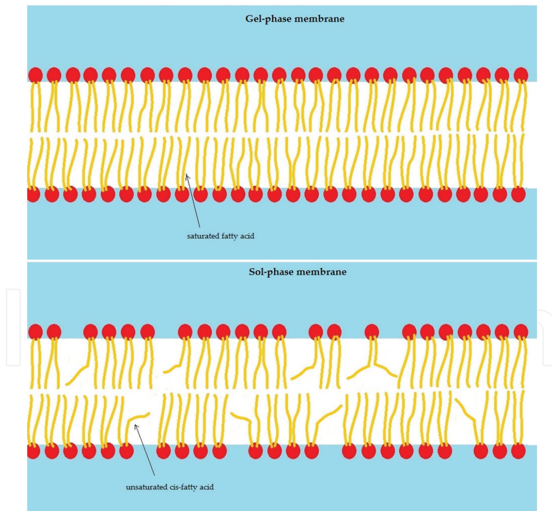
Figure 1. Different fluidity of cell membranes depending on the saturation of fatty acids: saturated fatty acids forming viscous membrane (up), unsaturated cis fatty acids forming fluid membrane (down).
