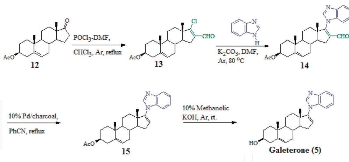
Figure 5. Synthesis of galeterone.
