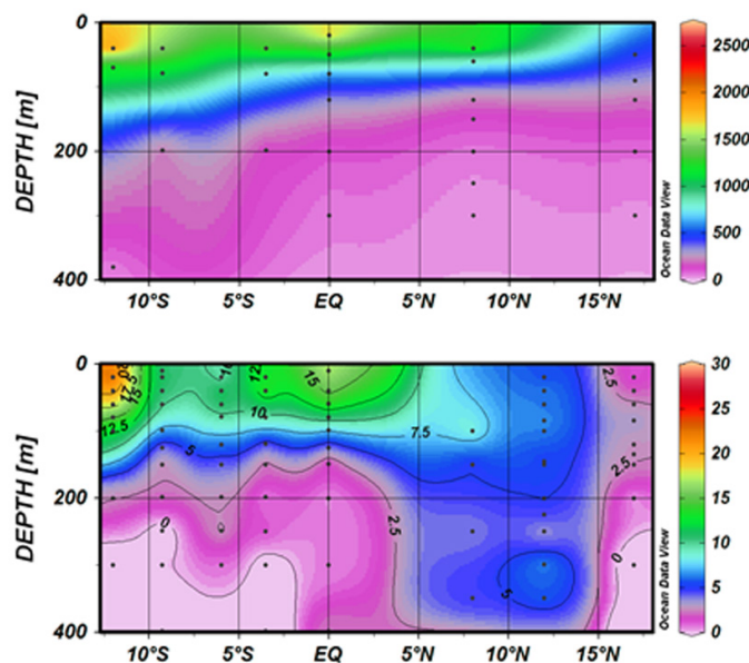
Figure 5-2 Distributions of the NiSOD metalloenzyme measured by targeted metaproteomics (top, fM) and particulate nickel (bottom, pM) across the central Pacific Ocean.
