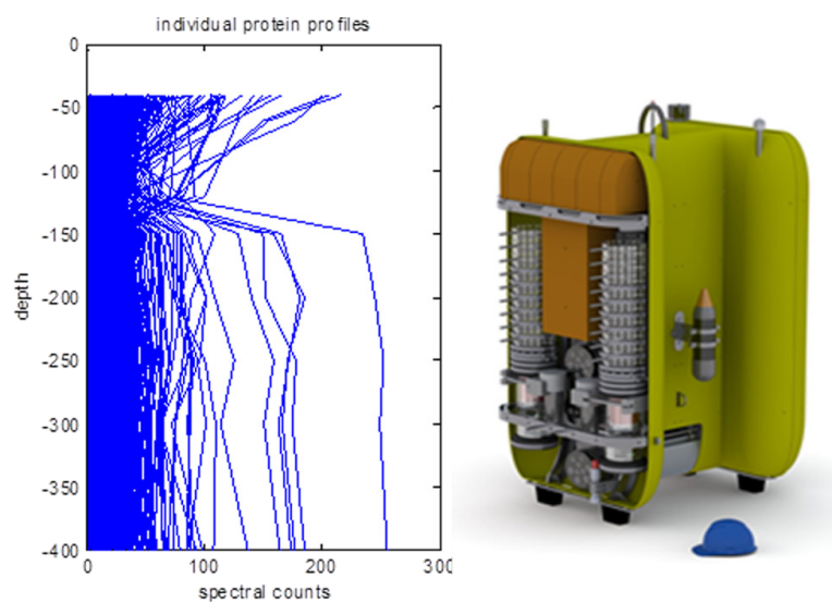
Figure 5-3 An example of several thousand proteins that can be measured simultaneously on a vertical profile through the Equatorial Pacific Ocean (left image). Design of autonomous underwater vehicle Clio with the shell removed to reveal micro-biome samplers (right image).
