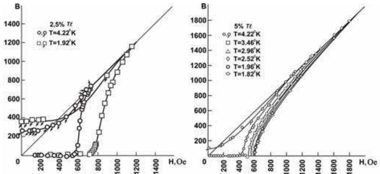
Fig. 17. The induction curve of long cylinders of single-crystals of alloys Pb+2,5wt% Tl; Pb+5wt% Tl (After Schubnikow et al., 1936).
