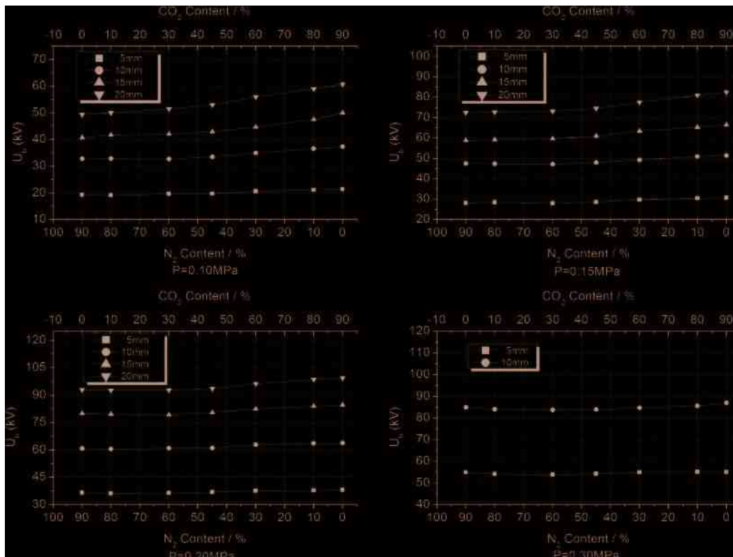
Figure 6. Relationship between AC-breakdown voltage and mixing contents of \text{c-C}_4\text{F}_8/\text{N}_2/\text{CO}_2 gas mixtures.
