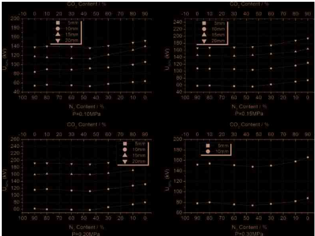
Figure 17. Relationship between positive lightning impulse breakdown voltage and mixing contents of \text{CF}_3\text{I} , \text{N}_2 , \text{CO}_2 gas mixtures.
