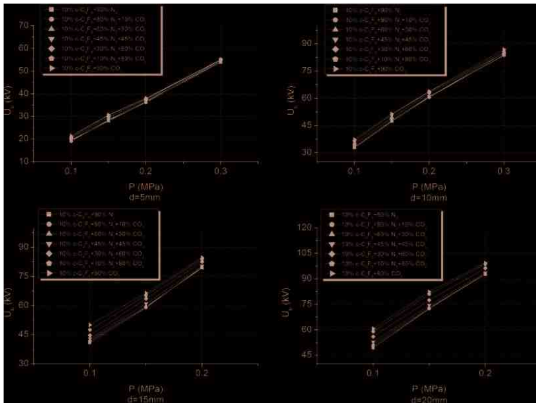
Figure 5. AC-breakdown voltage of \text{c-C}_4\text{F}_8/\text{N}_2/\text{CO}_2 gas mixtures with different electrodes gap distances.
