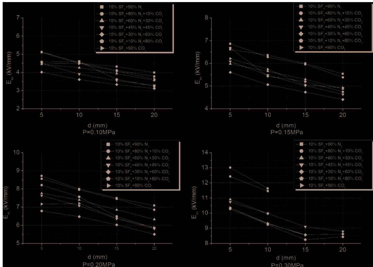
Figure A2. Maximum electric strength of SF 6 , N 2 , CO 2 gas mixtures with different gas pressures.
