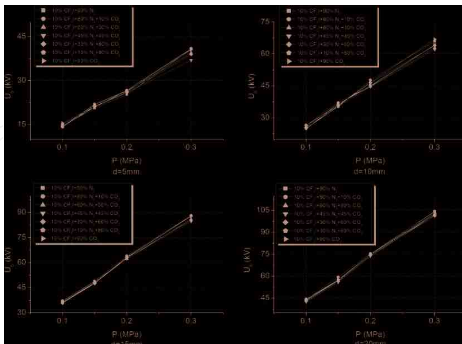
Figure 9. AC-breakdown voltage of CF_3I , N_2 , CO_2 gas mixtures with different electrodes gap distances.
