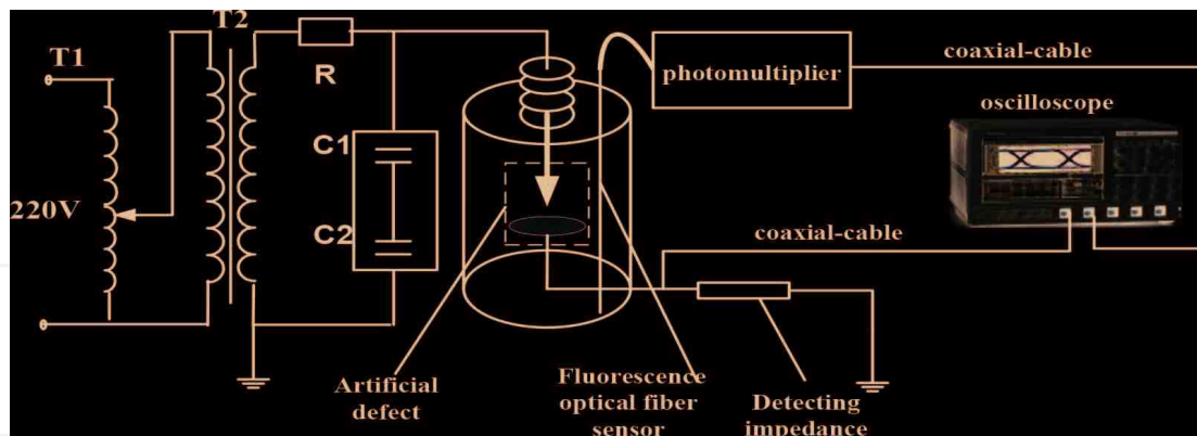
Figure 19. Figure of the fluorescent fiber sensor system.
