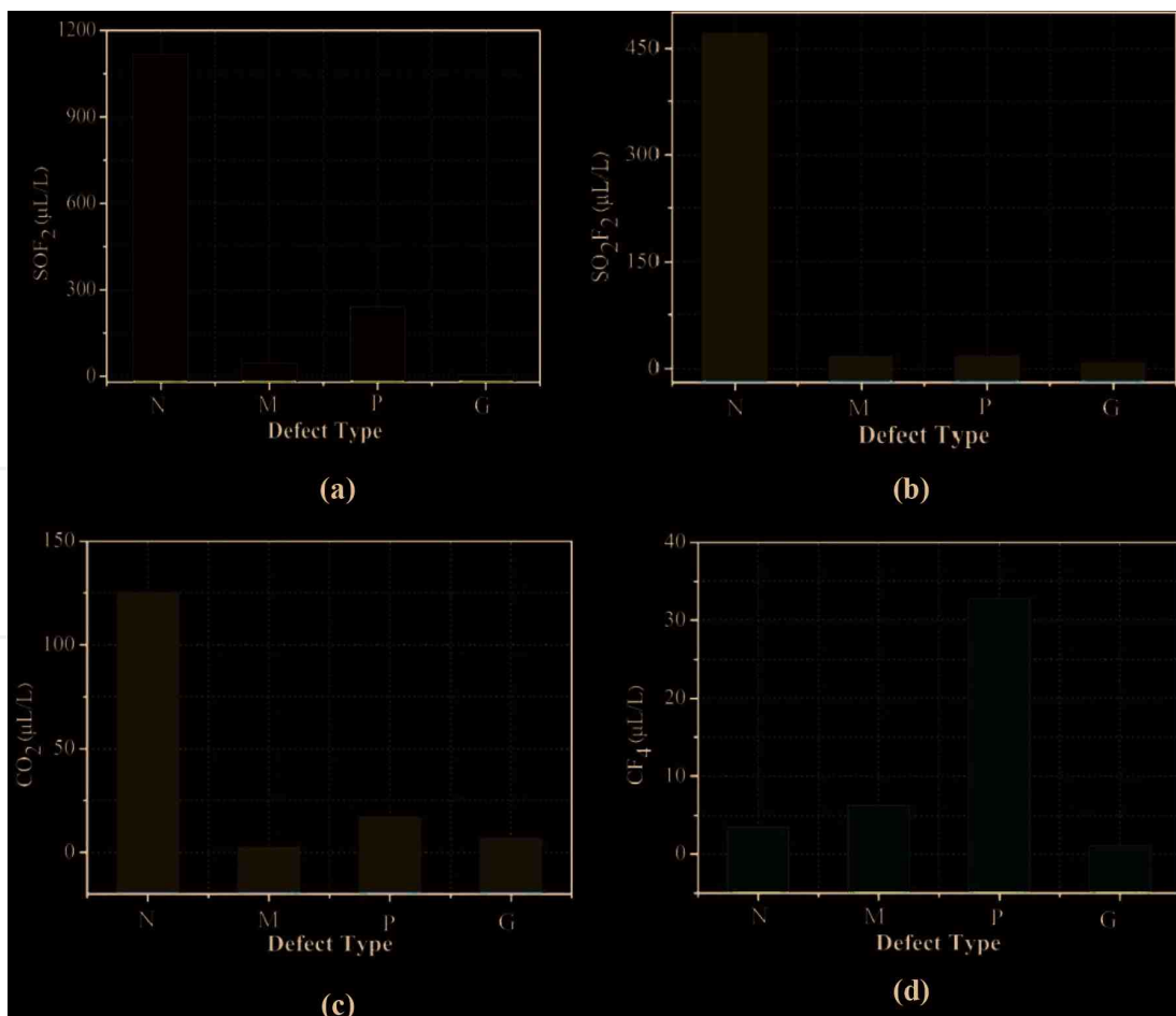
Figure 18. Decomposition components amount under four types of defects. (a) \text{SOF}_2 amount, (b) \text{SO}_2\text{F}_2 amount, (c) \text{CO}_2 amount, and (d) \text{CF}_4 amount.
