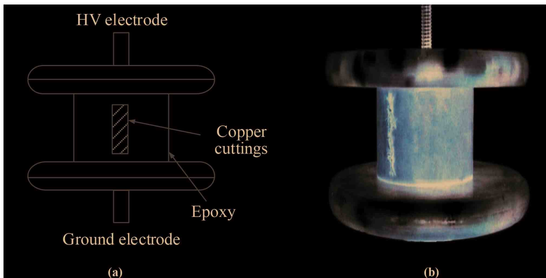
Figure 5. M-type insulation defect model. (a) Model diagram and (b) physical diagram.
