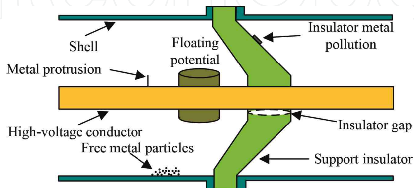
Figure 1. GIS internal insulation-defect type diagram.
