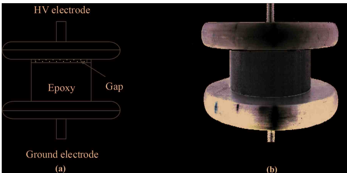
Figure 6. G-type insulation defect model. (a) Model diagram and (b) physical diagram.
