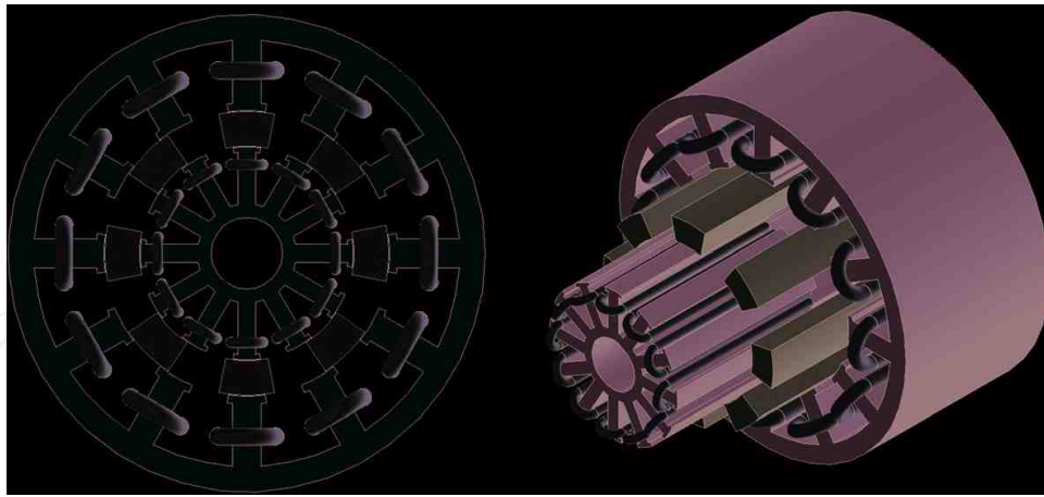
Figure 7. Three-phase 12/8-pole double-stator switched reluctance motor.
