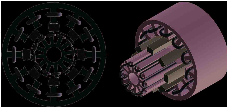
Figure 20. Three-phase 12/8-pole mechanical-offset double-stator switched reluctance motor.
