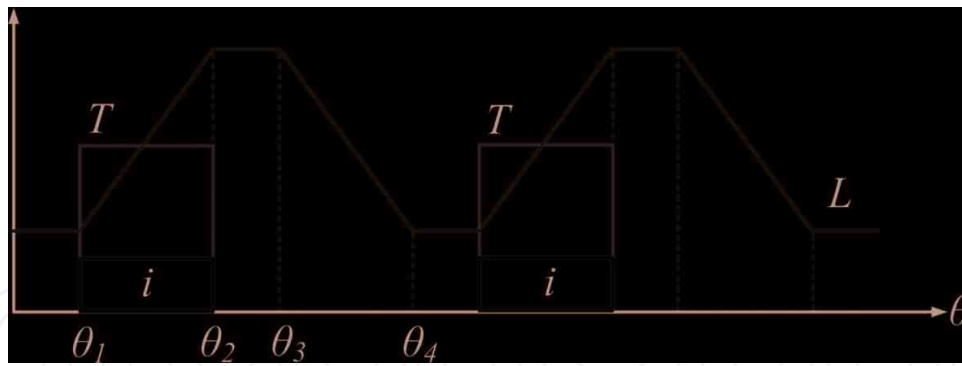
Figure 4. Theoretical operating waveform.
