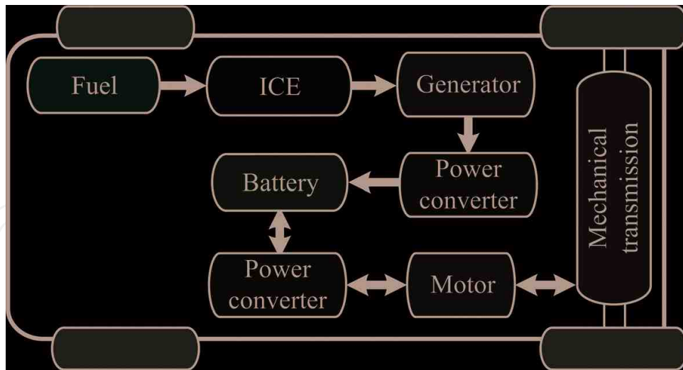
Figure 1. Series hybrid electric vehicle system.
