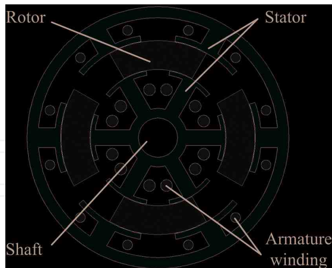
Figure 5. Three-phase 6/4-pole double-stator switched reluctance motor.
