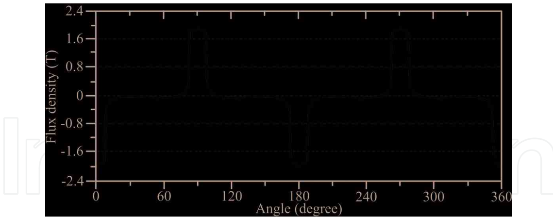
Figure 10. Airgap flux density of the switched reluctance motor.
