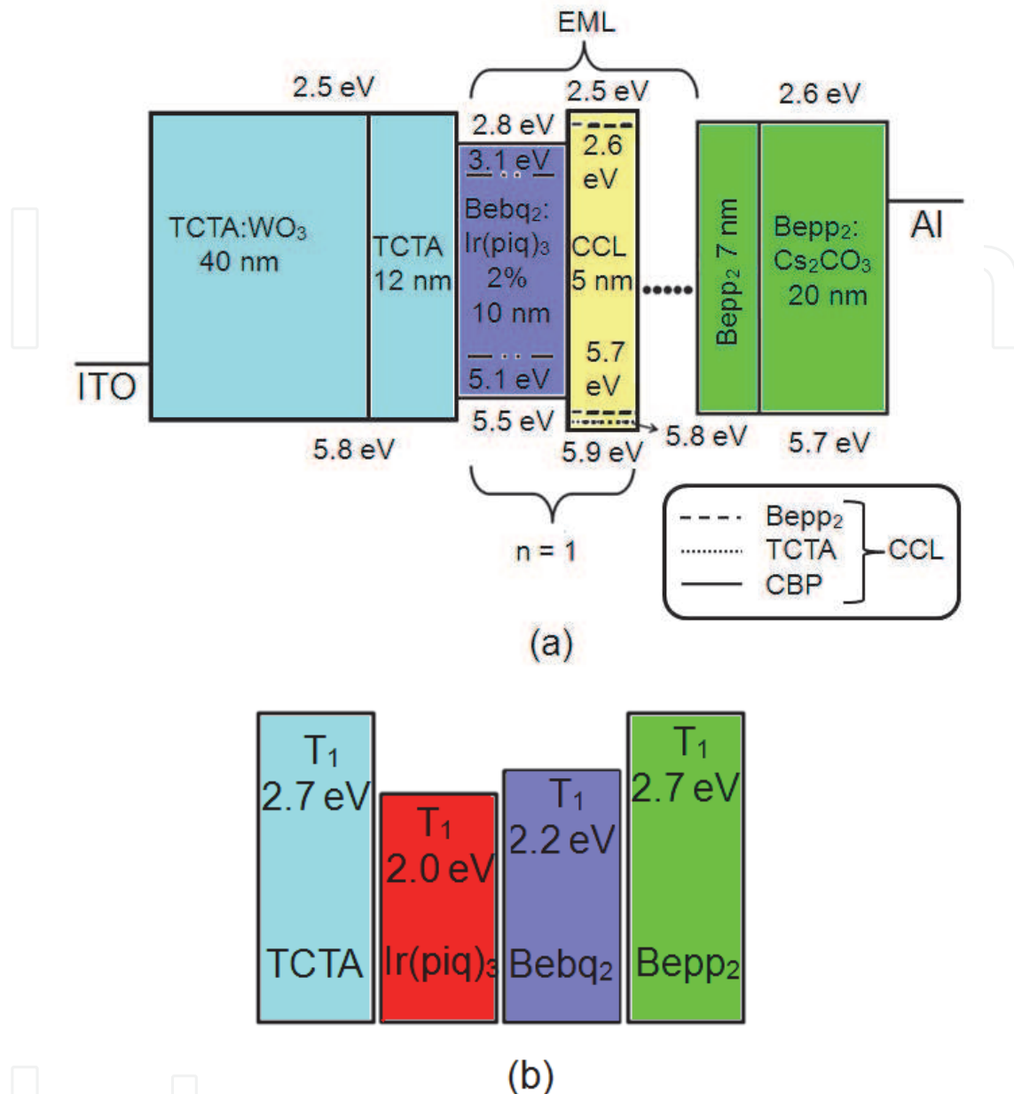
Fig. 3. (a) Energy band diagrams of fabricated red PHOLEDs with multiple quantum well structures. (b) Triplet energies of materials used in the present study.
