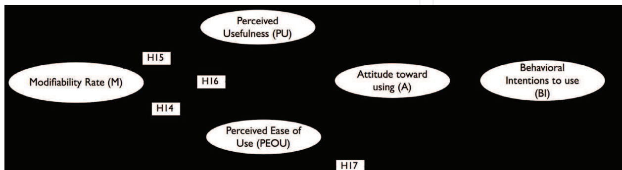
Fig. 7. Regression results for Modifiability Rate.
