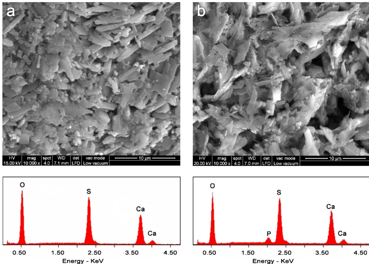
Figure 1. The micromorphology (SEM) of calcium sulfate-phosphate injectable cement. a) The set cement surface of unmodified low-dimensional medical grade calcium sulfate (crystal sizes less than 5 microns). b) The phosphate-containing material, which inhabits very small crystal formations grown into folding sheets. Energy dispersive (EDS) data, corresponding to the samples, are shown below each. The phosphorous content in the second sample is evident, whereas no separate phosphate phase appeared in XRD. The phosphate content resides as a substitution in the calcium sulfate crystals.
