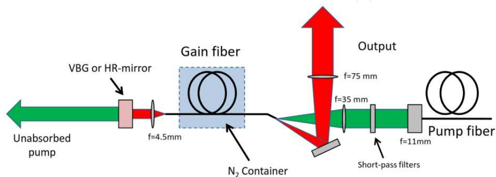
Figure 8. Cryogenically cooled fiber laser [64].
