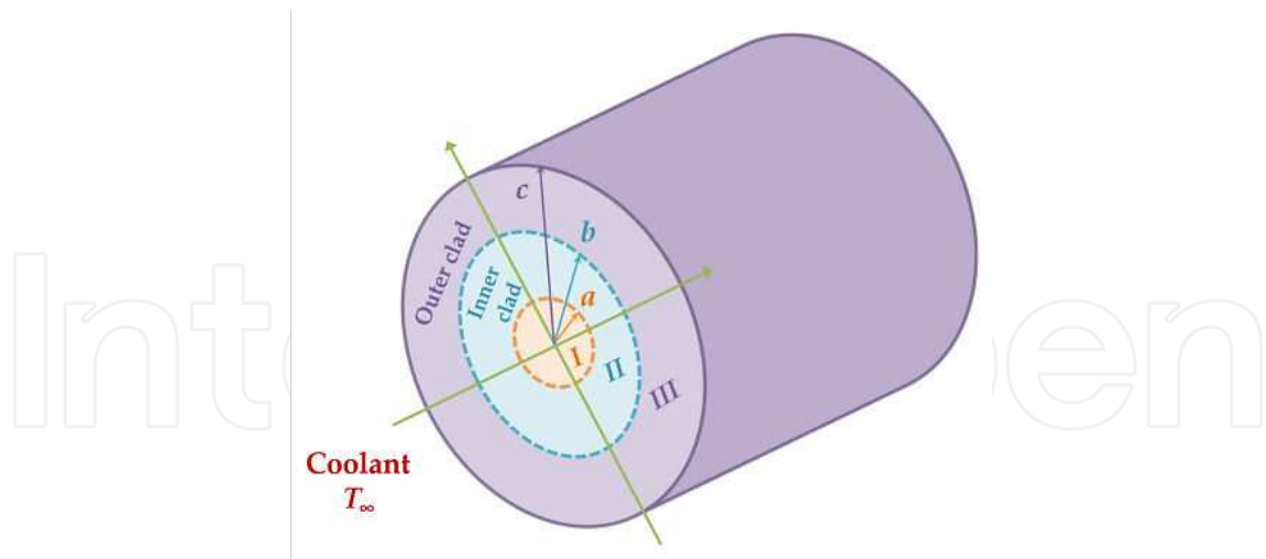
Figure 1. The geometry of various layers of a typical dual-clad fiber.
