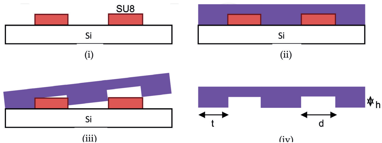
Figure 2. Process flow of PDMS stamps fabrication (i) SU8 master mold on silicon substrate (ii) PDMS prepolymer poured on SU8 (iii) peeling off PDMS replica after curing (iv) fabricated PDMS stamp.
