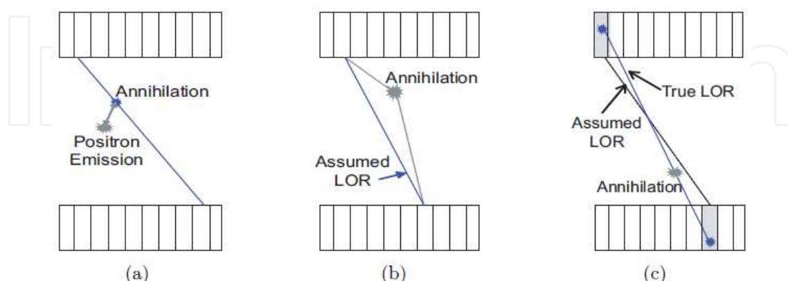
Figure 1. Schematic drawings of some of the effects that degrade spatial resolution in PET: a) the positron range, b) the acolinearity effect and c) the Depth of Interaction effect or parallax error.
