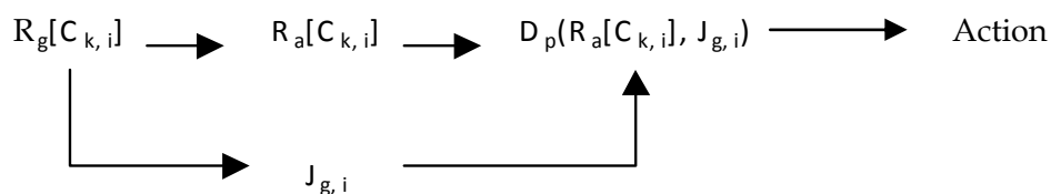
Fig. 7. Grouping-Focusing and Searching loop
