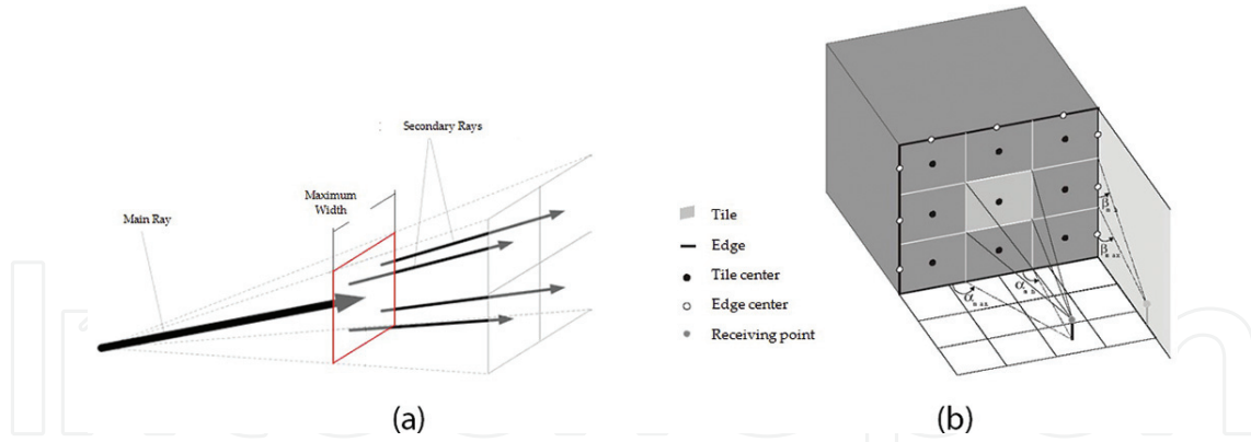
Figure 7. The division of the rays in the RT method [12] (a) and the geometry of the intelligent method of ray tracing IRT [10].
