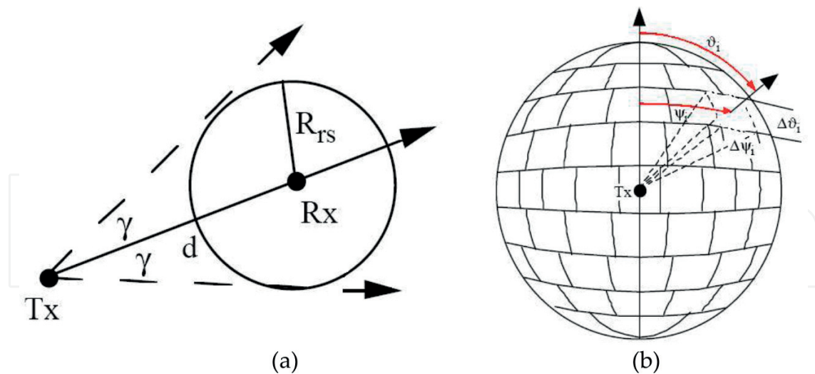
Figure 6. Cross-section of the receiving sphere (a) and rays launching method concept (b) [11].
