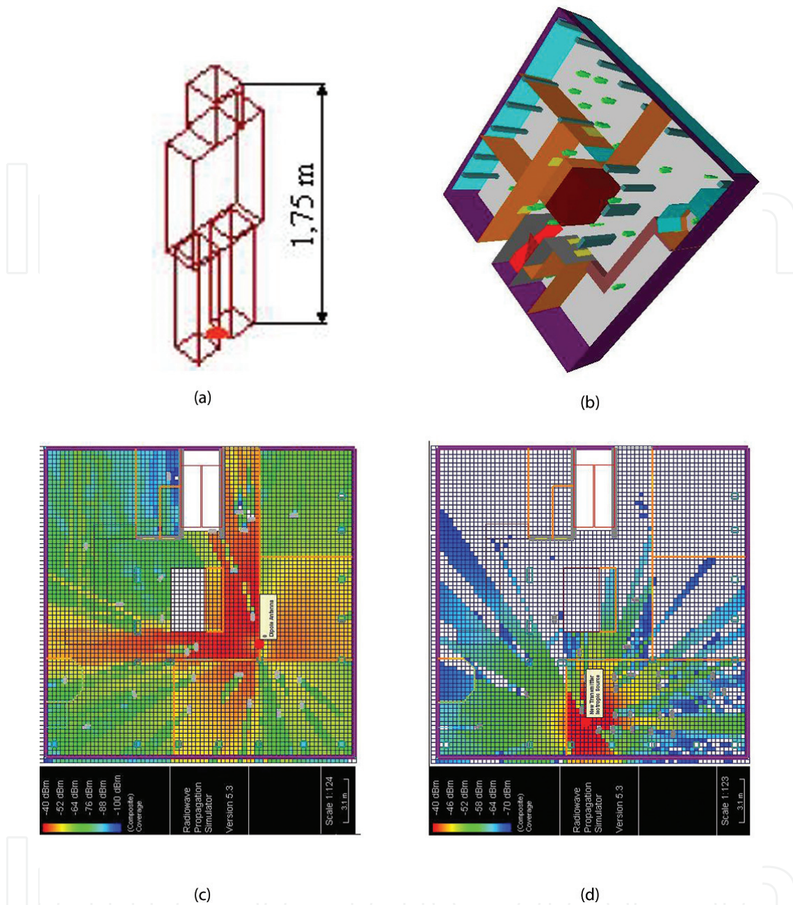
Figure 16. The deployment of several human models (a) on the ground floor (b) of the C-5 to simulate their effect on the extent of IEEE 802.11 g (c) and Bluetooth networks (d).
