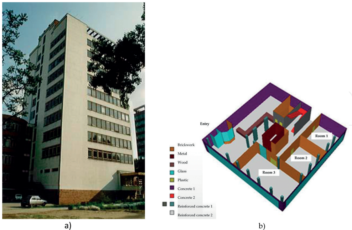
Figure 12. Photo of the Wrocław University of Science and Technology building C-5 (a) and the numerical model of the ground floor with use of defined construction materials an example (b).
