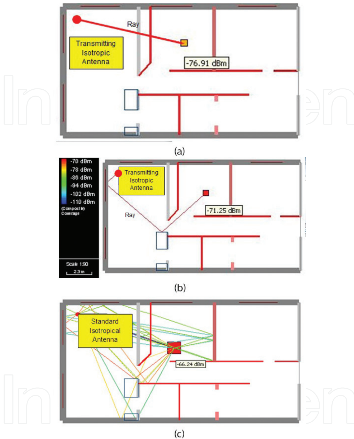
Figure 4. Simulation results obtained using: only the direct radius (nonlinear of M-W model) (a), of the strongest ray (the dominant path D-P model) (b), and ray tracing, 3D RT, approach (c).
