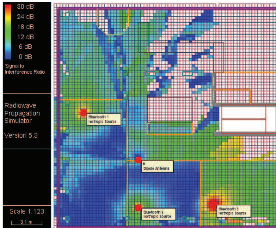
Figure 15. Levels of interference between Bluetooth and IEEE 802.11 g systems on the ground floor of the C-5 building.
