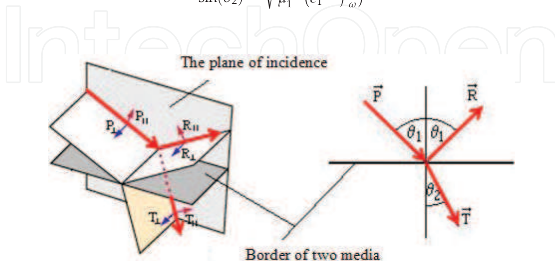
Figure 8. The EM wave reflection and transmission phenomenon.
