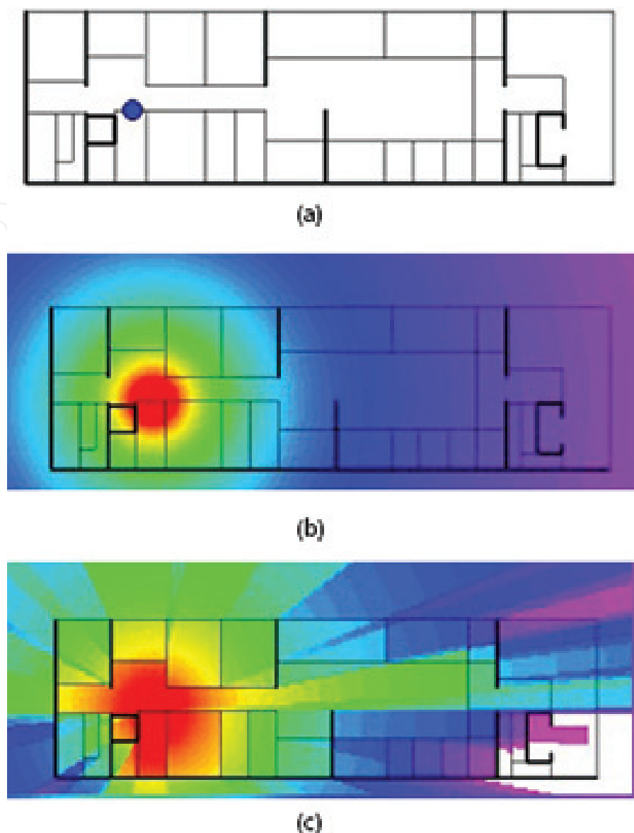
Figure 2. The projection of floors and location of the access point (a), the distribution of the signal for one-slope model (b), and for nonlinear model of multi-walls (c) [3].
