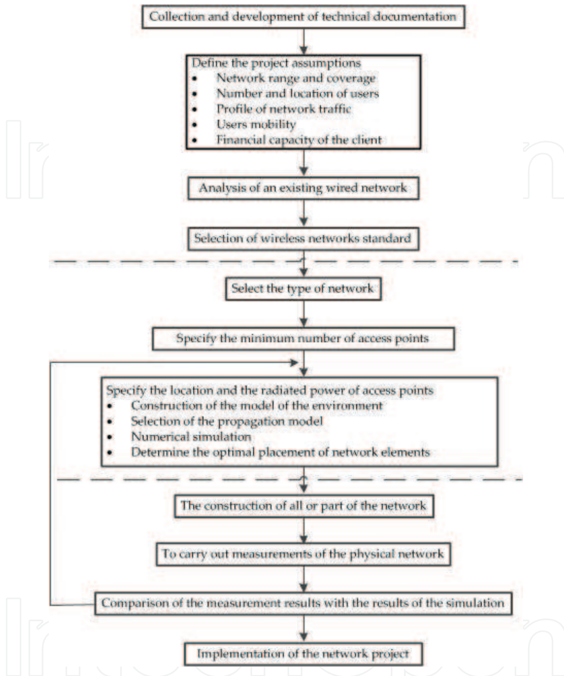
Figure 11. Design algorithm of wireless communication networks.
