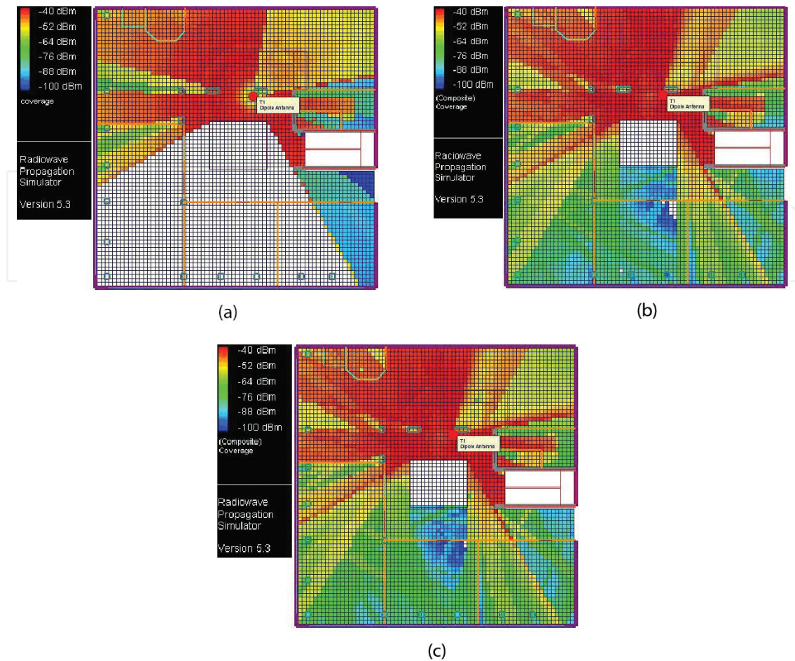
Figure 13. The simulation results of signal power distribution in a MW model (a), the 2.5 D RT model (b), and the 3D RT model (c) for radiated power 10 dBm at f = 2.45 GHz on the ground floor of building C-5 of WRUoS&T.
