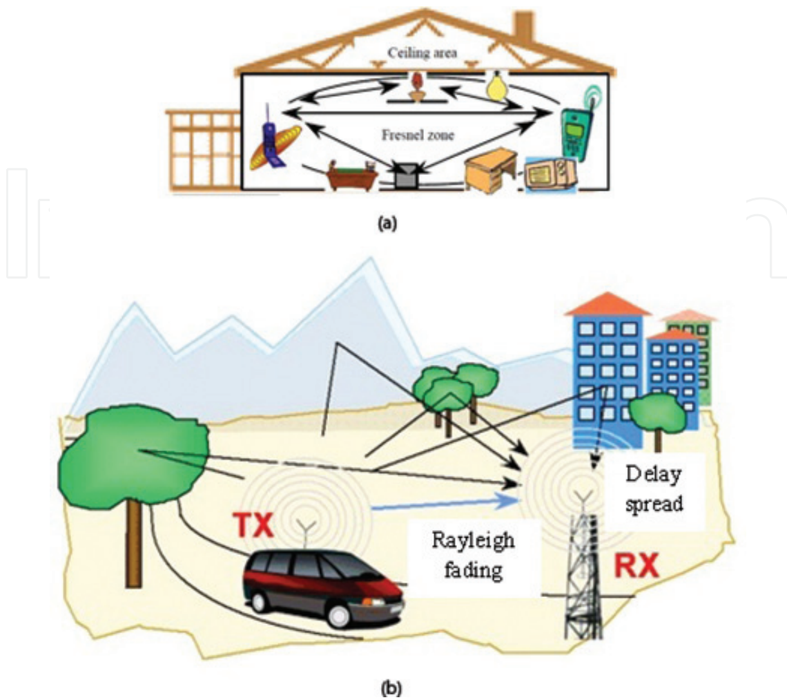
Figure 1. Wireless systems impairments in: indoor (a) and outdoor (b) environments.
