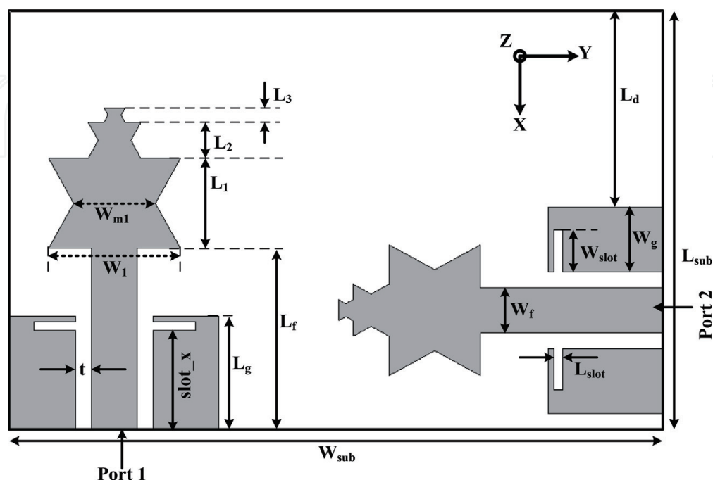
Figure 1. Geometry of the antenna.
