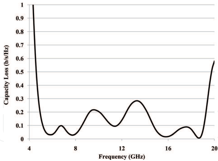
Figure 16. Capacity loss versus frequency characteristic.
