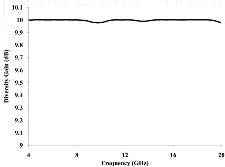
Figure 15. Diversity gain versus frequency characteristic.
