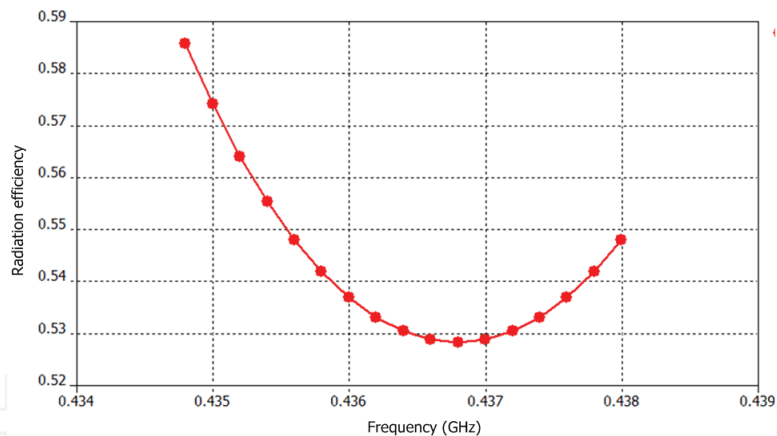
Fig. 20. Broadband variation in the radiation efficiency of the CSPP-1 antenna.
