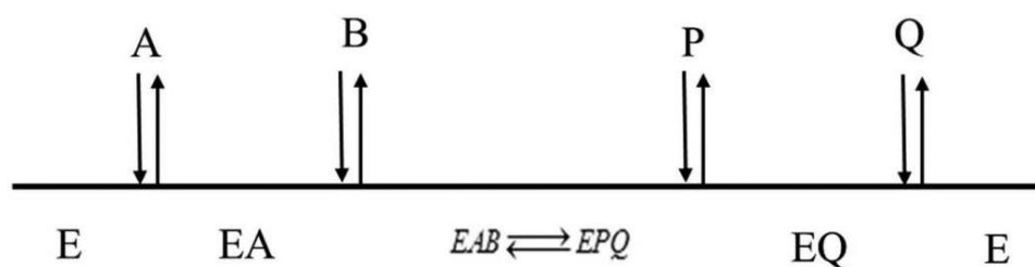
Figure 3. Ordered sequential mechanism.
