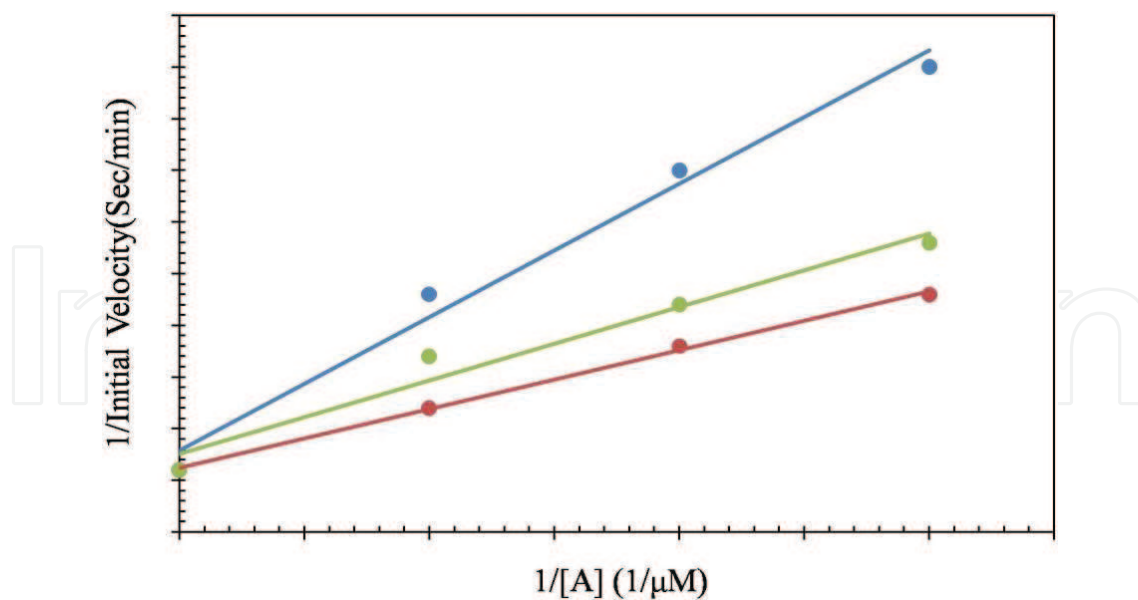
Figure 6. Double reciprocal plot for double-displacement mechanism (at different levels of B).
