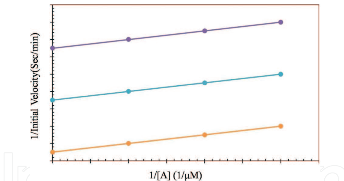
Figure 7. Double reciprocal plot for double-displacement mechanism (at different levels of B).
