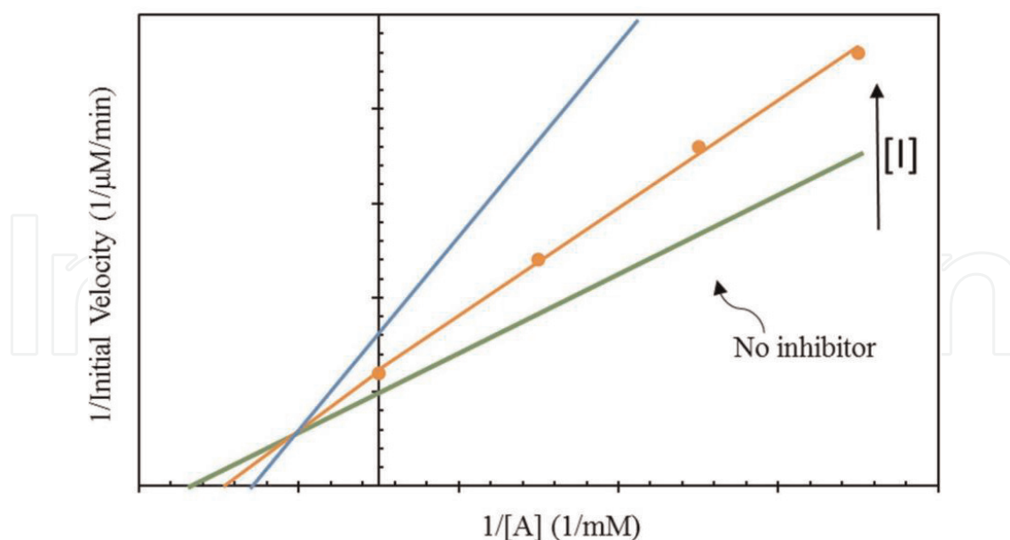
Figure 14. Graphical representation of noncompetitive inhibition.
