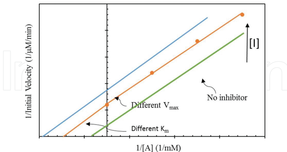
Figure 13. Graphical representation of uncompetitive inhibition.
