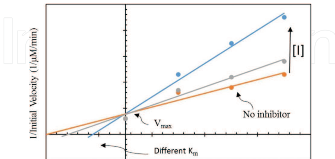
Figure 12. Graphical representation of competitive inhibition.
