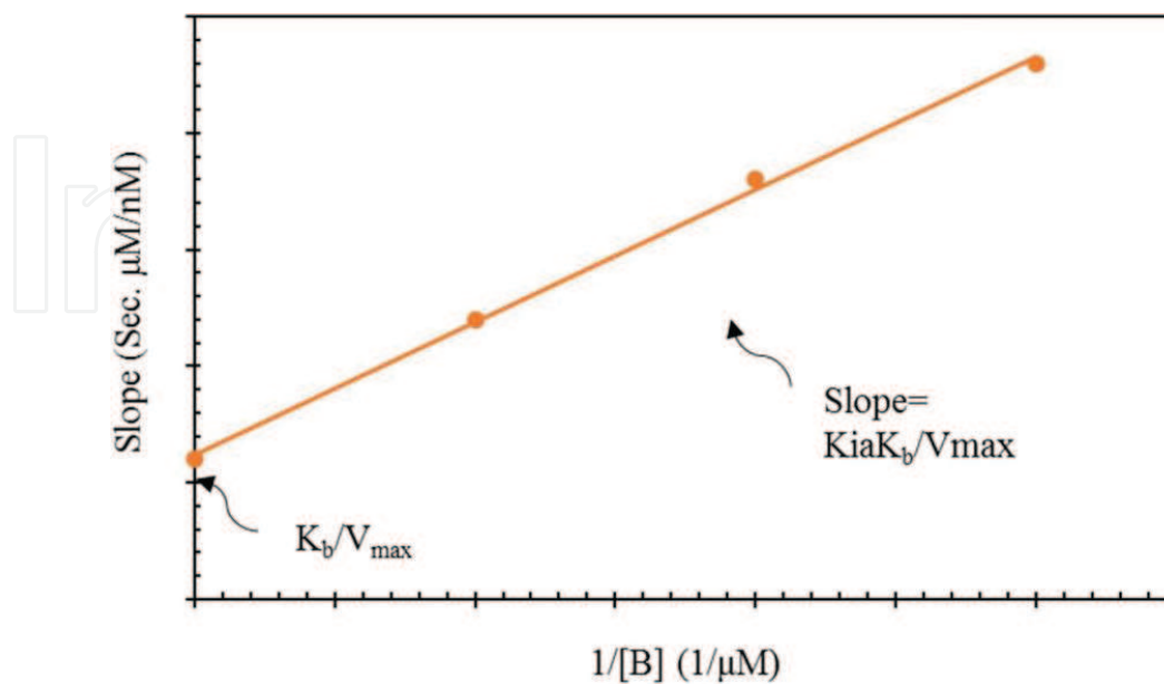
Figure 16. Secondary plot of slope versus reciprocal of concentration of B .
