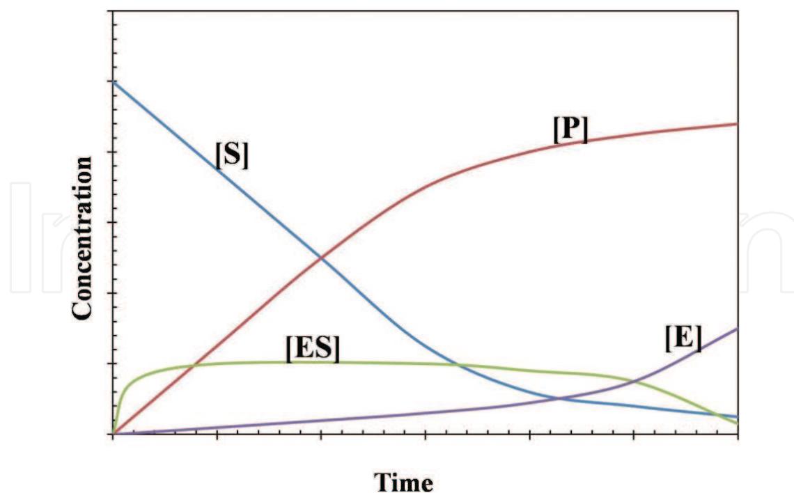
Figure 1. Progress curve for simple enzyme for catalysed reaction [7].
