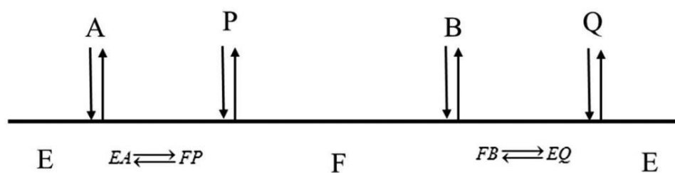
Figure 4. Random sequential mechanism.
