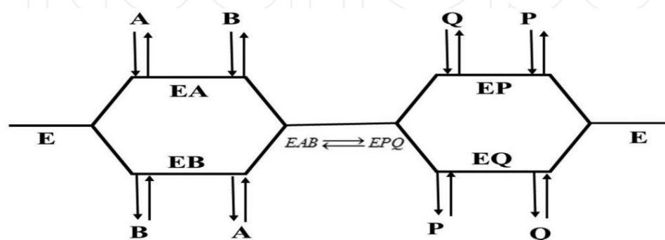
Figure 5. Double-displacement reaction mechanism.
