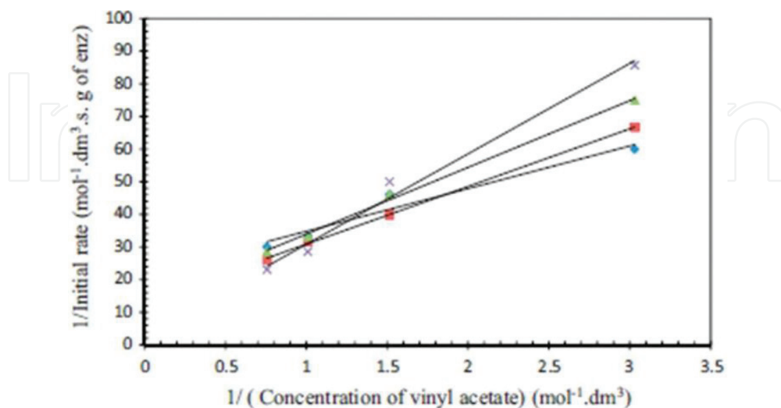
Figure 8. Lineweaver Burk plot of initial velocity versus concentration of vinyl acetate.
