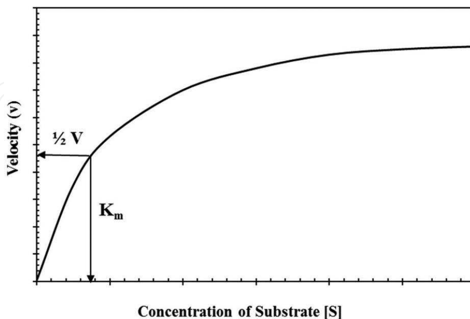
Figure 2. Initial velocity of reaction versus the concentration of substrate [4].
