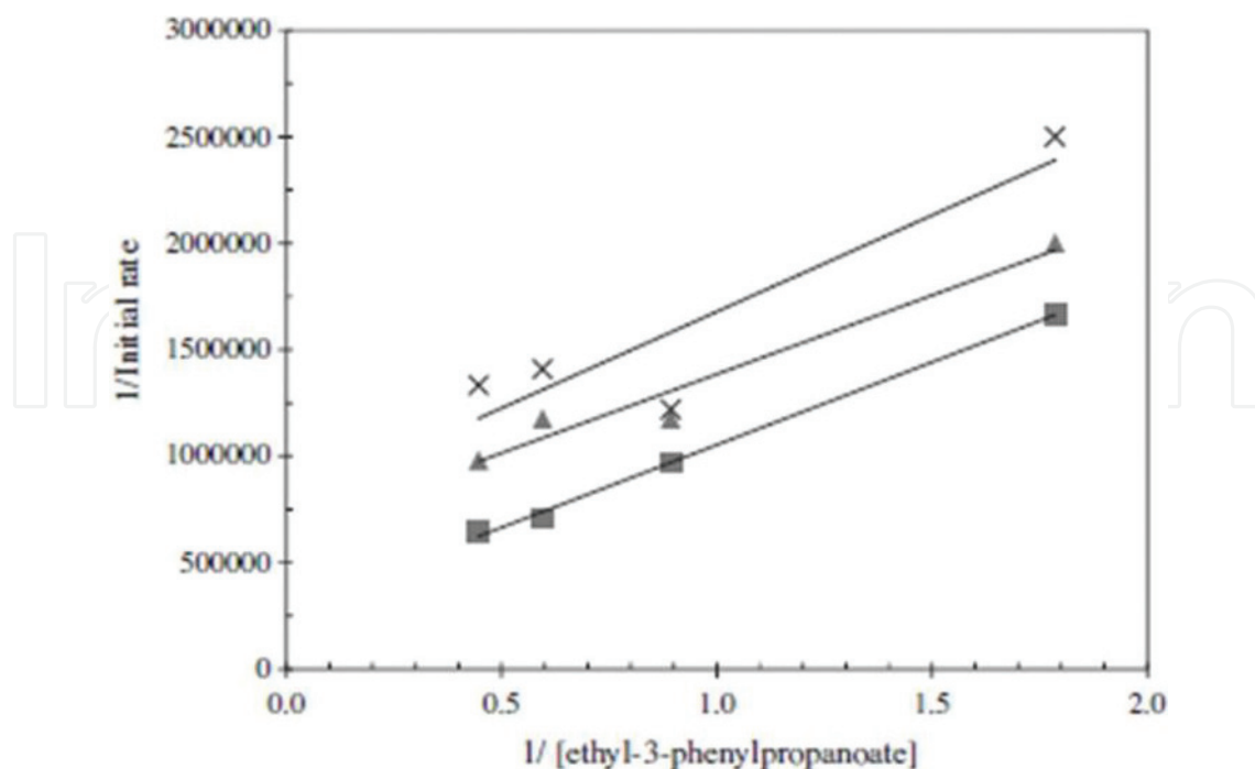
Figure 9. Lineweaver Burk plot of initial velocity versus concentration of ethyl-3-phenylpropanoate.
