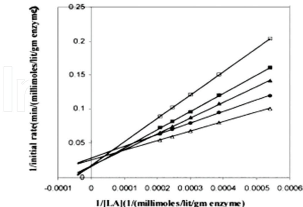
Figure 10. Lineweaver Burk plot of initial velocity versus concentration of lauric acid.
