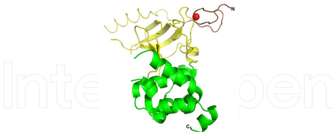
Figure 10. Spatial structure of the RFTS domain from human Dnmt1 (PDB code: 3epz). \beta -Barrel is colored in yellow, \text{Zn}^{2+} -binding motif – in brown, \alpha -helical bundle – in green. \text{Zn}^{2+} ion is shown as a red sphere.
