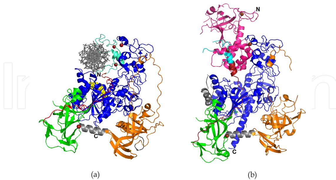
Figure 9. Spatial structure of murine Dnmt1. (a) Dnmt1(650–1602) complexed with AdoHcy and a 19 bp DNA duplex containing two unmethylated 5′-CG-3′/3′-GC-5′ sites (PDB code: 3pt6). (b) Dnmt1(291–1620) in apo-form (PDB code: 3av4). The RFTS, CXXC, BAH1, BAH2, and MTase domains are colored in magenta, cyan, green, orange, and blue, respectively. Zn 2+ ions are in red and AdoHcy is in yellow, both in space-filling representation. DNA is in grey, in sticks representation. The autoinhibitory linker CXXC–BAH1 is colored in red. The borders of the domains are shown according to [9].
