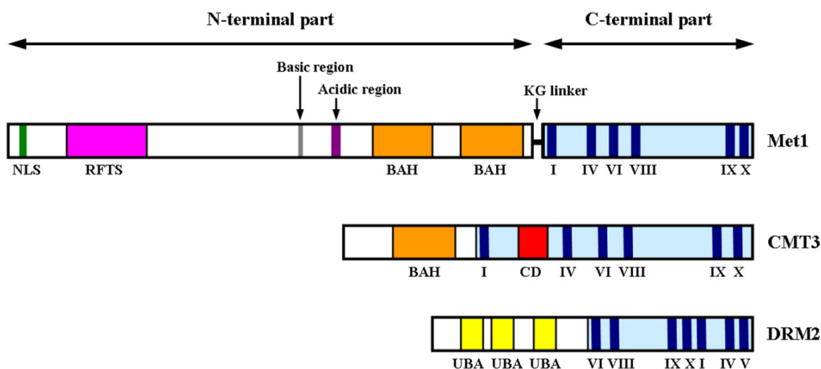
Figure 15. Domain architecture of different C5-DNA MTases from A. thaliana . Met1 – MTase similar to mammalian Dnmt1, CMT3 – chromomethyltransferase 3, DRM2 – MTase with the circular permutation of conservative motifs. The catalytic domains are marked by a light blue filling. The other domains are signed in the bottom. Roman numerals indicate the conservative motifs of C5-DNA MTases.
