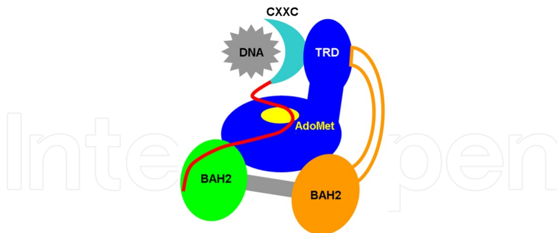
Figure 12. A model of the Dnmt1 autoinhibition mechanism in maintenance DNA methylation. The domains are colored as in Figure 9. The CXXC domain and the autoinhibitory linker (in red) close the active center of the enzyme. Additionally, the BAH2–TRD loop (in orange) keeps the TRD away from the DNA.
