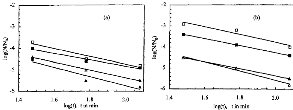
Figure 6. Effect of applied chlorine and contact time on survival of (a) total coliform and (b) total count. □ Cl 2 , 1.2 mg/L; ■ Cl 2 , 2.0 mg/L; △ Cl 2 , 1.8 mg/L; ▲ Cl 2 , 0.9 mg/L. (Adapted from Chiang et al. [25])
