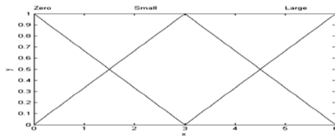
(a) Innovation mean value ( \bar{v} )
