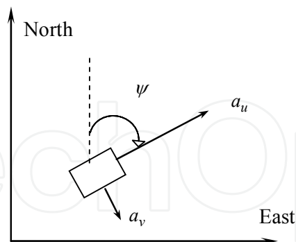
Fig. 3. Two-dimensional inertial navigation, Farrell & Barth (1999)
