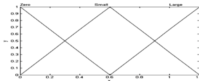
(c) Threshold c
