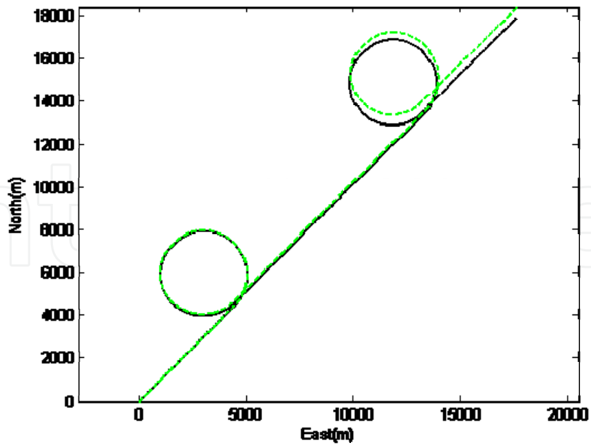
Fig. 5. Trajectory for the simulated vehicle (solid) and the INS derived position (dashed)
