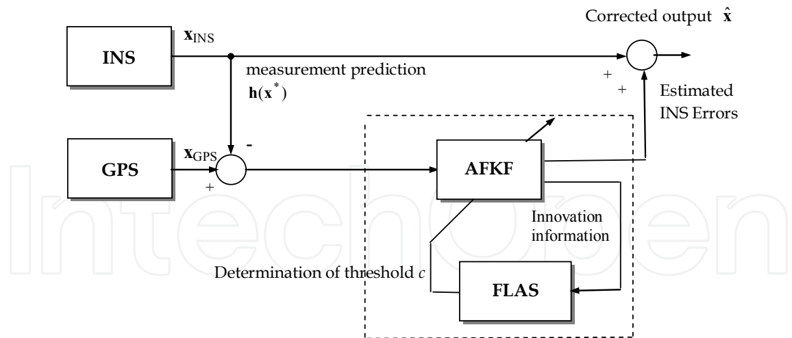
Fig. 4. GPS/INS navigation processing using the FAFKF for the illustrative example 1.
