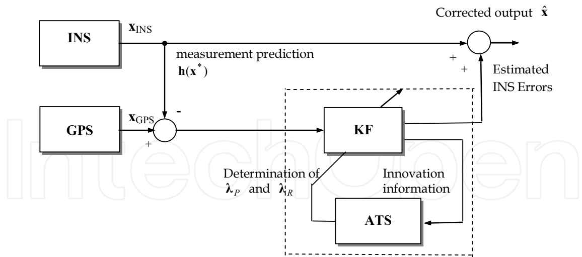
Fig. 10. GPS/INS navigation processing using the IAE/AFKF Hybrid AKF for the illustrative example 2
