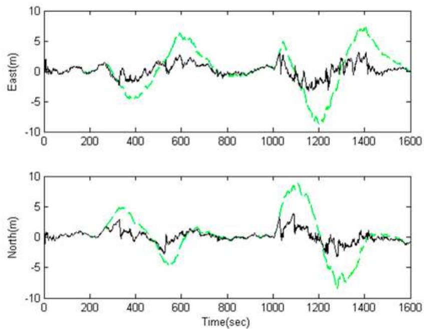
Fig. 8. Navigation accuracy comparison for AFKF and FAFKF
