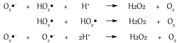
Figure 1. Reaction mechanism of superoxide radical.
