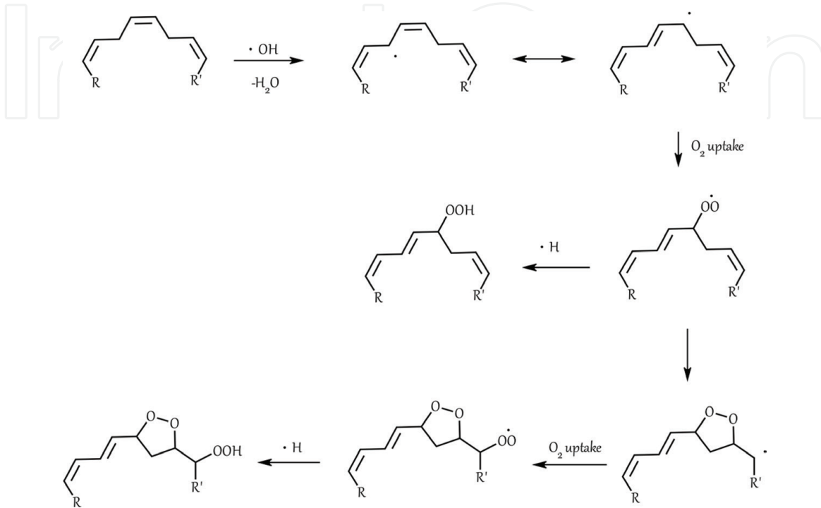
Figure 2. Reaction of hydroxyl radical with polyunsaturated fatty acids.
