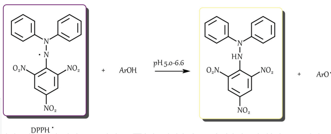
Figure 12. DPPH• reduction by an antioxidant.
