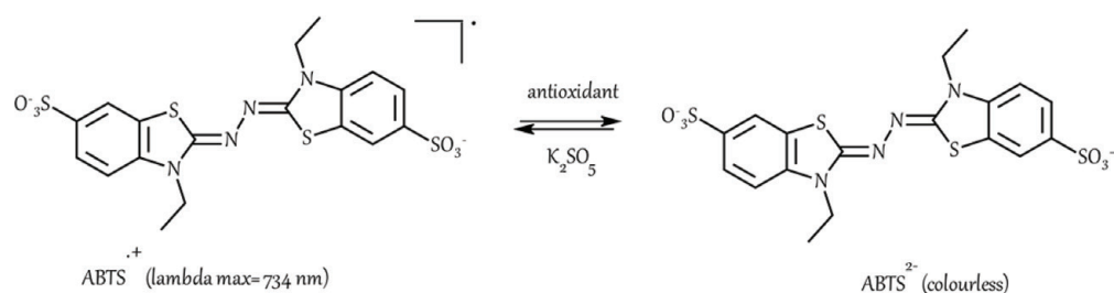
Figure 14. Reaction of ABTS •+ with antioxidant compounds.
