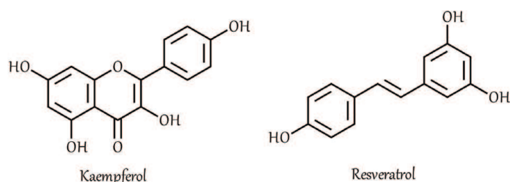
Figure 7. Phenolic compounds with ability to SET.
