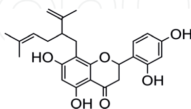
Sophoraflavanone G
