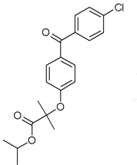
Fenofibrate (5) Isopropyl 2-[4-(4-chlorobenzoyl) phenoxy]-2-methyl propanoate
