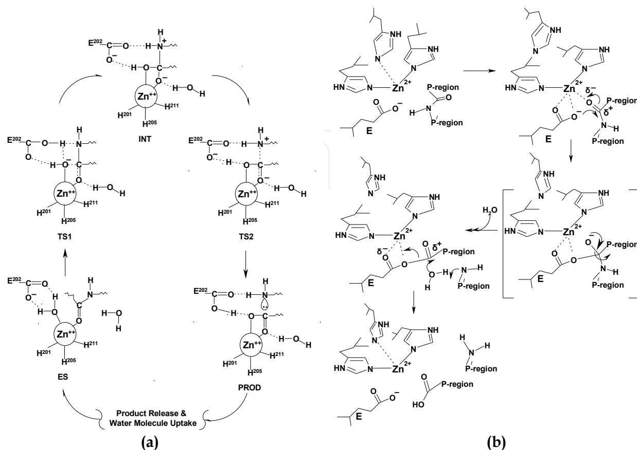
Fig. 6. Matrix metalloproteases: initially, Zn^{2+} is three-coordinated and continues as penta-coordinated either (a) with three H^{\delta 2} -nitrogens, the P_1 -carbonyl oxygen and one H_2O -oxygen or (b) with two H^{\delta 2} -nitrogens, the P_1 -carbonyl oxygen and two oxygens of catalytic E-residue (modified from Pelmeshnikov & Siegbahn, 2002).
