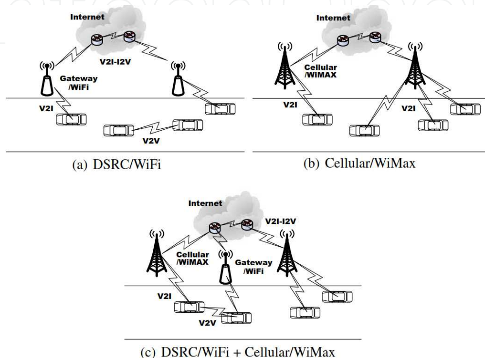
Fig. 2. Wireless vehicular networking scenarios.
